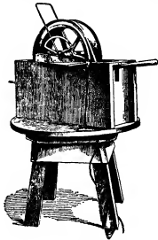
FIG. 7.—Marvin Kite Reel for hand power.
