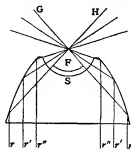
FIG. 46.—Wenhem's Paraboloid Condenser.
