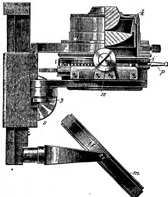
FIG. 42.—Abbe Illuminating Apparatus with Ordinary Condenser (Zeiss).
