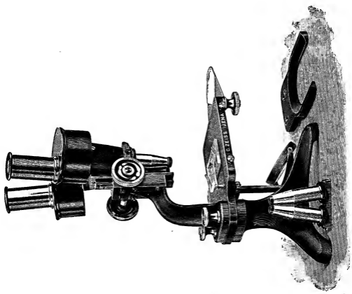
FIG. 59.—GREENOUGH'S BINOCULAR MICROSCOPE (ZEISS).
