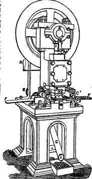
FIG. 3.—Cutting Machine.
