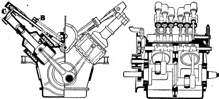
FIG. 20.—The Bentley Eight-cylinder Diagonal Tandem-compound Superheated-Steam Engine.
