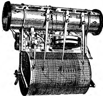
FIG. 8.—Marvin Kite Meteorograph.
