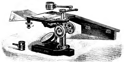
FIG. 57.—LARGE DISSECTING STAND (ZEISS).
