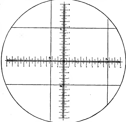
Greenwich Astrophotographic Catalogue, vol. 1, by permission of the Controller of H.M. Stationery Office. FIG. 16.—Diagram of the diaphragm in eyepieces of the micrometer used for measuring the plates of the Astrophotographic Catalogue.
