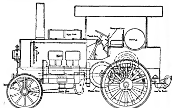
FIG. 37.—45 h.p. Thornycroft Military Oil Tractor.
