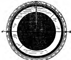
FIG. 3.—Abbe's Marine Nephoscope. Horizontal Projection of Mirror.
