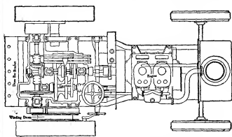
FIG. 36.—Marshall's 30 h.p. Agricultural Tractor.
