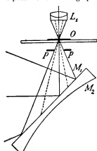
FIG. 40.—Mirror Illumination.
