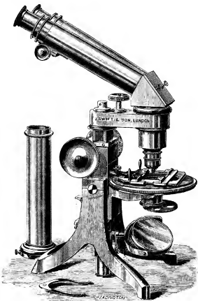
FIG. 58.—STEPHENSON'S BINOCULAR MICROSCOPE (SWIFT).
