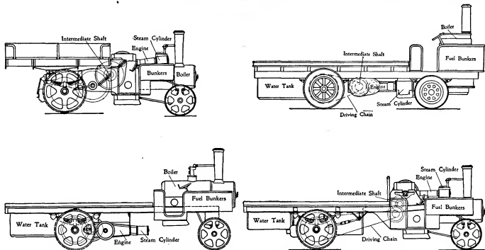
FIGS. 6-a.—Standard and Representative Types of Present-day Steam-wagon Construction.
