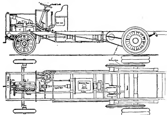
FIG. 29.—A typical Six-ton Petrol Wagon Chassis, by Commercial Cars, Ltd., Luton.
