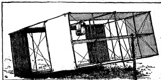
FIG. 6.—Marvín-Hargrave Kite, with Meteorograph in position.
