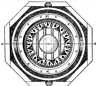
FIG. 4.—Abbe's Marine Nephoscope. Horizontal Projection of Compass.
