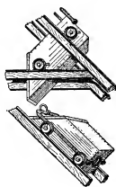
FIG. 18.—Ore and water skips for inclined shaft. Alls-Chalmers Co., Milwaukee, Wisconsin, makers.
