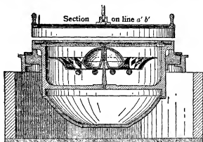
FIG. 5.—Abbe's Marine Nephoscope. Vertical Section.
