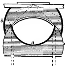
FIG. 47.—Siedentopf's Cardioid Condenser.
