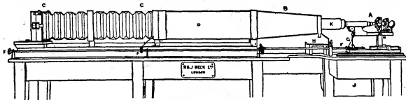
Micrographic Apparatus.
