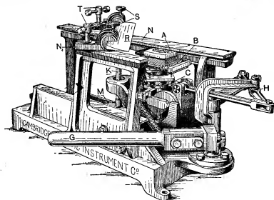
Large Sliding Microtome.
