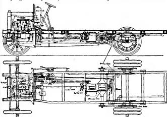
FIG. 27.—The well-known 16 h.p. Two-ton Albion Chassis.
