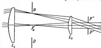
FIG. 38.—Huygenian Eyepiece.
