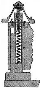
FIG. 51.—Micrometer Screw Adjustment of Leitz.
