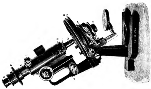
FIG. 61.—PETROGRAPHICAL MICROSCOPE (ZEISS).
