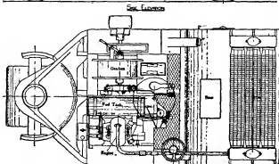
FIG. 35.—One of Barford & Perkins's Water-ballast Rollers. XVIII. 30
