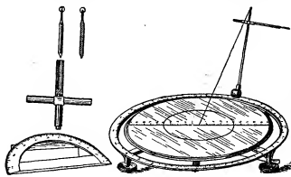
FIG. 2.—Marvin's Nephoscope.
