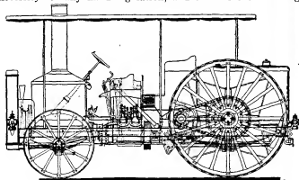
FIG. 26.—Colonel Crompton's Superheated Steam Tractor.
