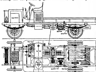
FIG. 24.—The Sheppey "Steam-gas" or Superheated Steam Vehicle.
