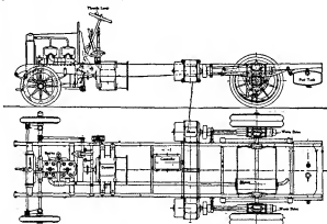
FIG. 32.—The Hallford-Stevens Petrol-electric Chassis.
