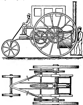
FIG. 1.—Trevehick's Steam Carriage of 1802: side view and plan.
