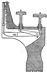
FIG. 53.—Double Lever Adjustment of Watson & Sons.
