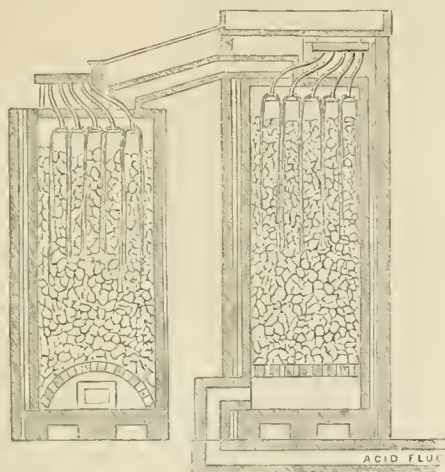
Fig. 3.—Section of Coke Towers for condensing the Hydrochloric Acid Gas.
