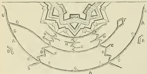
Fig. 2.—Siege Works.
