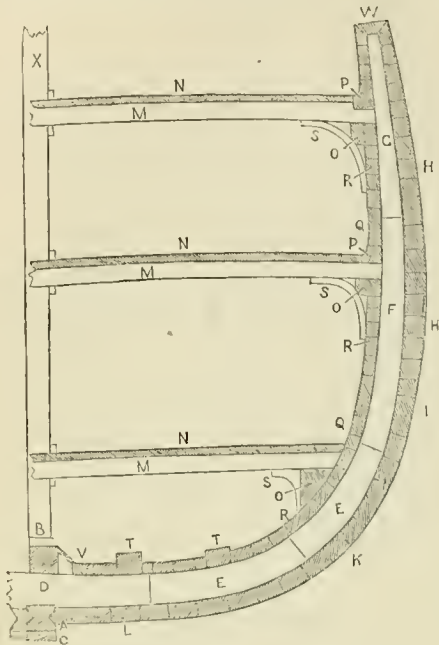
Fig. 9.—Rib and Decks in section.
