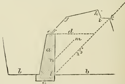
ac , revêtment; b , bottom of ditch, level of ground within the work; d , top of rampart; fgh , parapet; ik , banquette; ikl , mass of earth supported by revêtment; m , centre of gravity of mass; n , point of greatest pressure on revêtment.
