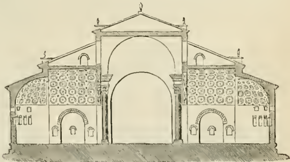
Fig. 3.—Transverse Section of Basilica of Maxentius. (From Fergusson's Hand-book of Architecture .)
