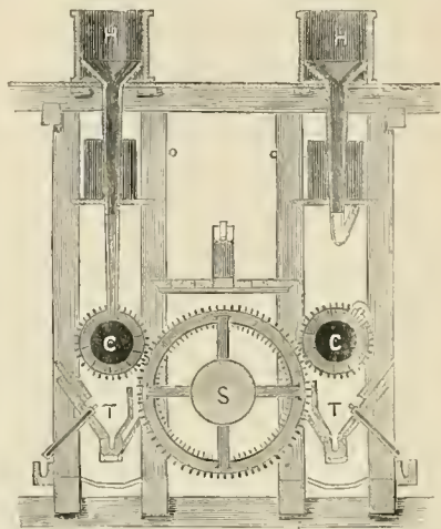
Fig. 2.—Vertical Section of Amalgamating Apparatus.
