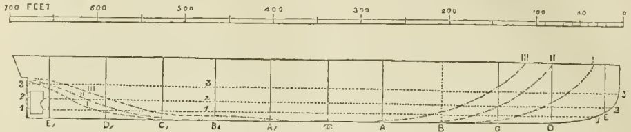
Fig. 1.— Great Eastern —Sheer Plan.
