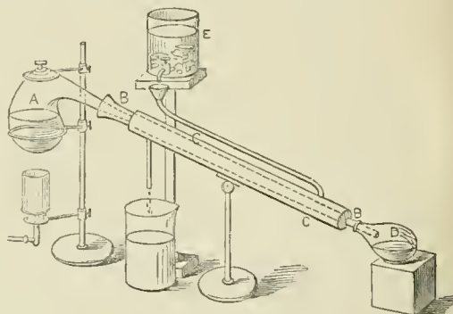
Liebig's Condenser.
