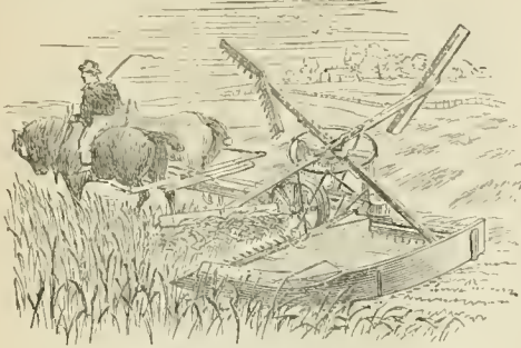
Fig. 3.—Samuelson's Self-delivery Reaping-machine.
