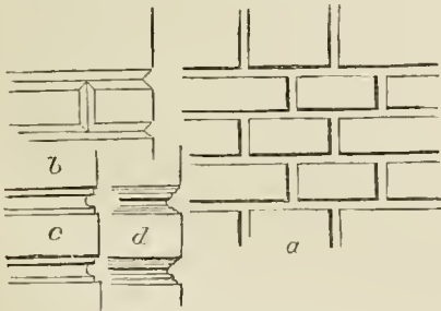
Rustication.
