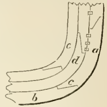
Fig. 7.—Stem. a, stem; b, keel; c, boxing d, apron; e, stantion.
