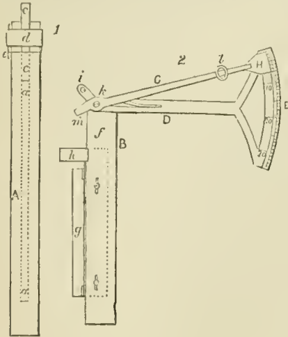
Daniell's Pyrometer.
