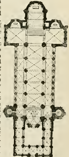
Fig. 1.—Plan of Church at Laach.
