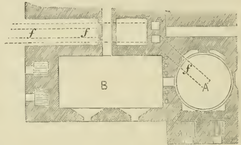
Fig. 2.—Plan of Decomposing Furnace.
