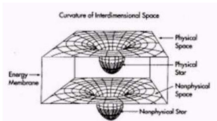
Embedding of an uncollapsed spherical star.
