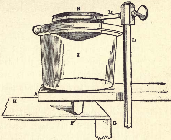
FIG. II. CROOKES' APPARATUS.
