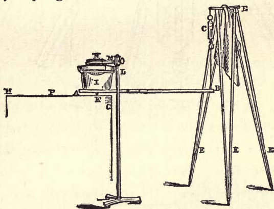
FIG. 9. CROOKES' APPARATUS.
