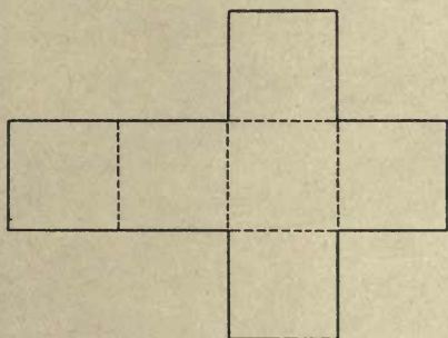
CUBE.
