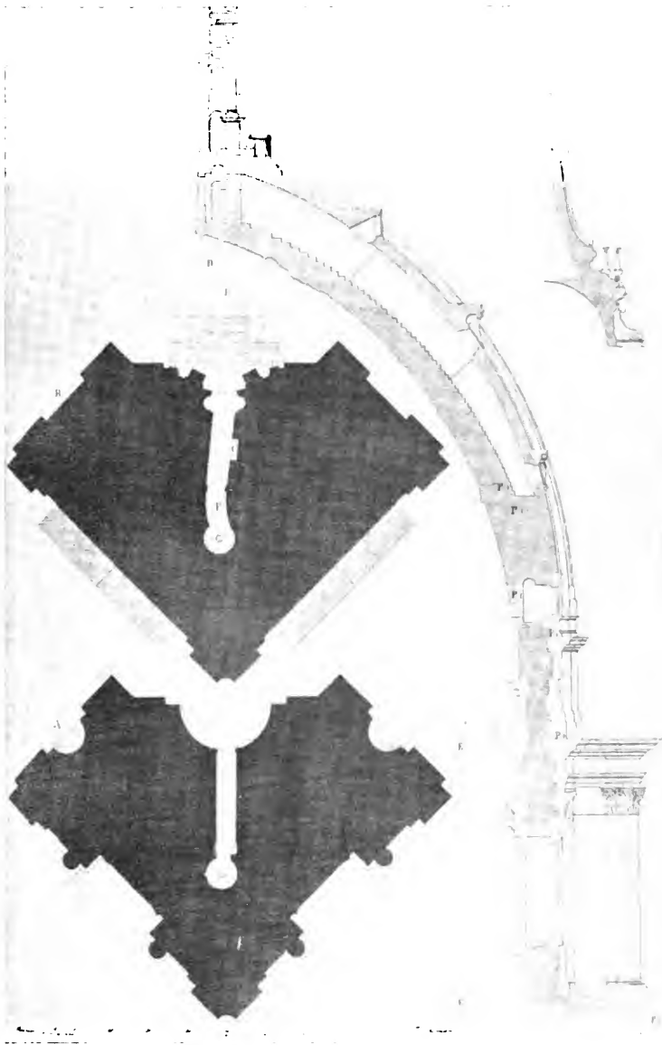
St. Peter's. Plan showing how the Dome and the Shrine Galleries of its piers are ascended.—From Pistoletti's "Il Vaticano."
