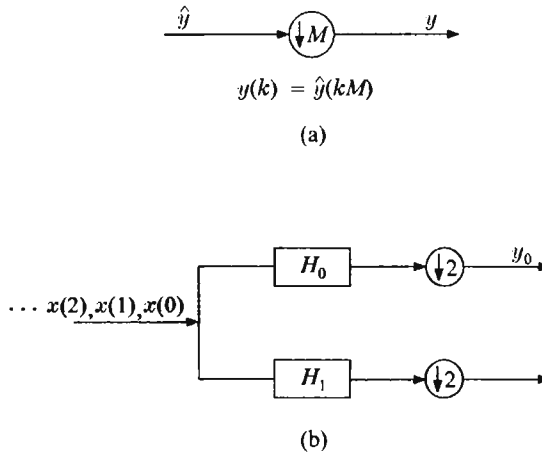
FIGURE 6.4: (a) Subsampling operation and (b) filtering interpretation of the Haar transform.
