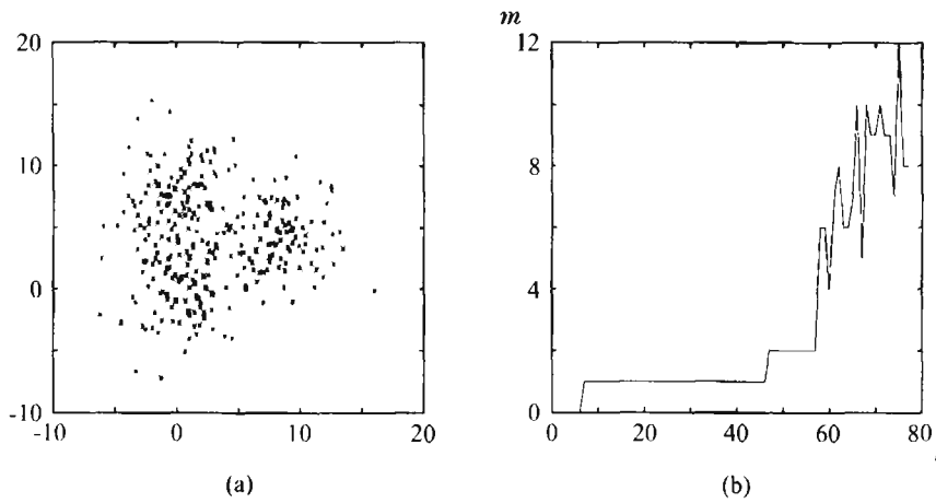
FIGURE 16.3: (a) Three overlapped clusters. (b) The plot of m versus r .
