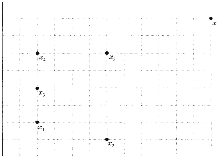
FIGURE 11.8: The setup of Example 11.10.
