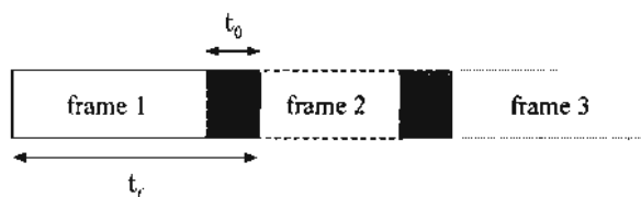
FIGURE 8.6: Successive overlapping frames for the computation of the DFT feature vectors.
