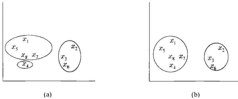
FIGURE 12.3: (a) The clustering produced by the MBSAS. (b) The clustering produced by the TTSAS.
