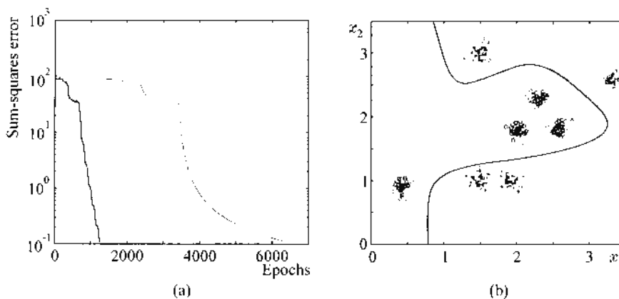
FIGURE 4.15: (a) Error convergence curves for the adaptive momentum and the momentum algorithms. Note that the adaptive momentum leads to faster convergence. (b) The decision curve formed by the multilayer perceptron.
