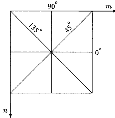
FIGURE 7.2: The four orientations used to construct co-occurrence matrices.
