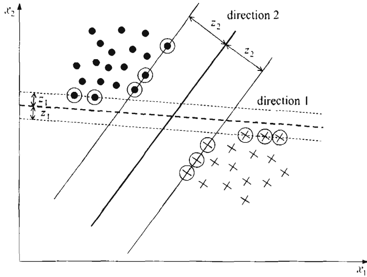
FIGURE 3.8: The margin for direction 2 is larger than the margin for direction 1.
