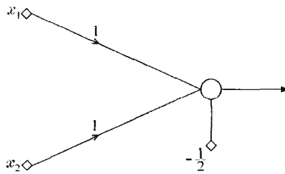
FIGURE 4.3: A perceptron realizing an OR gate.
