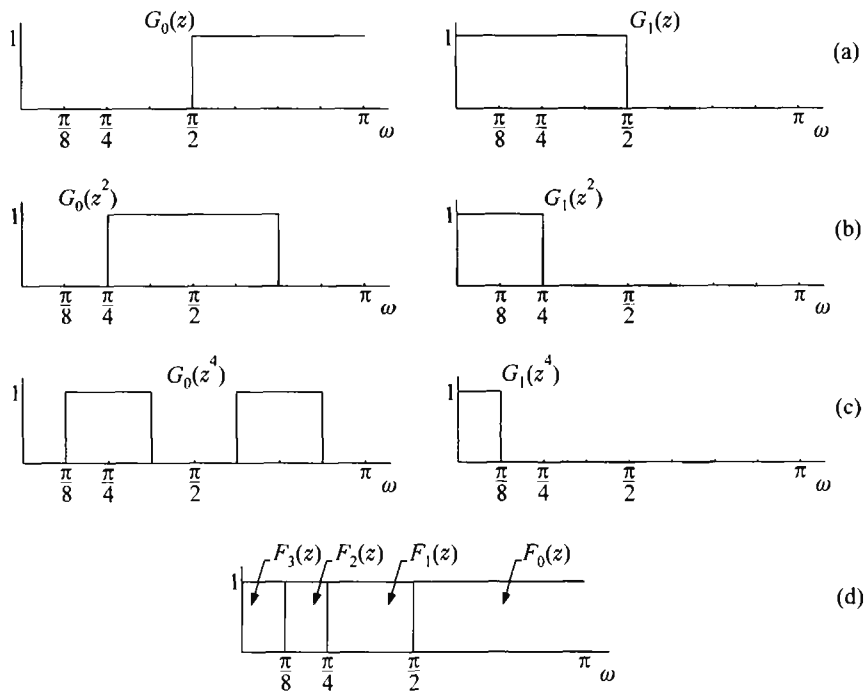
FIGURE 6.14: Filter bandwidths in an octave band filter bank.
