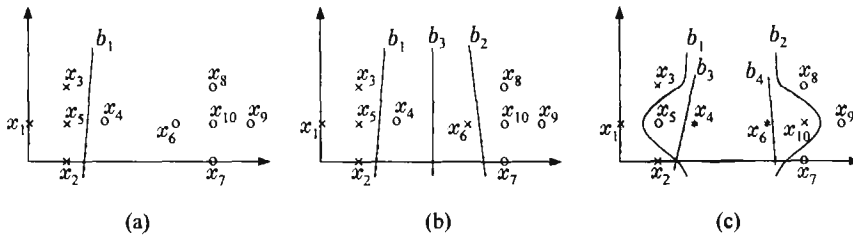
FIGURE 15.16: (a) The setup of Example 15.7(a). (b) The setup of Example 15.7(b). (c) The setup of Example 15.7(c).
