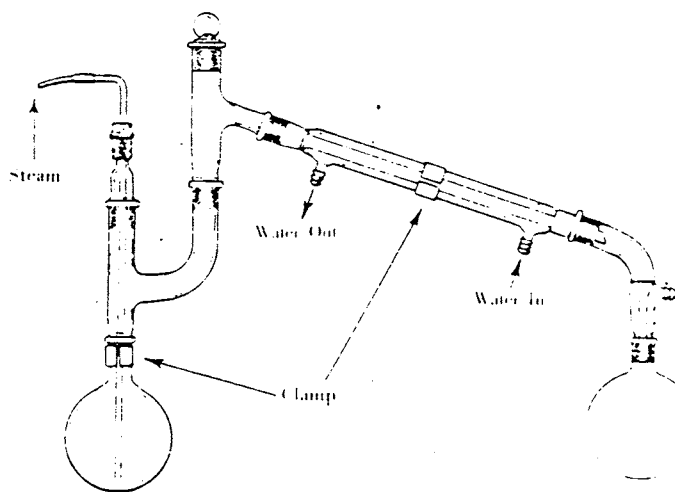
Steam Distillation
