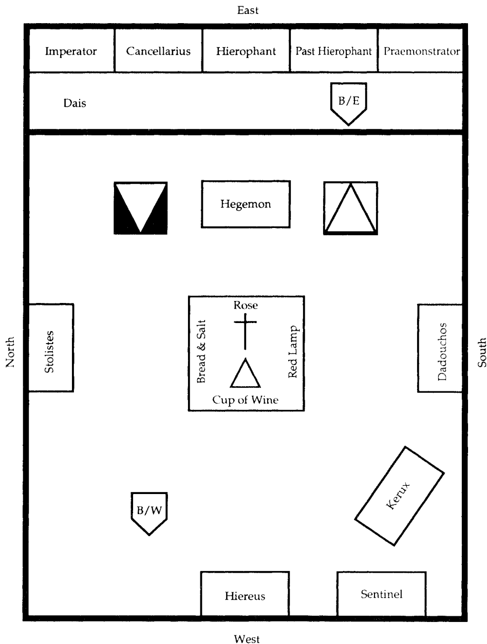
Figure 1 Temple Layout
