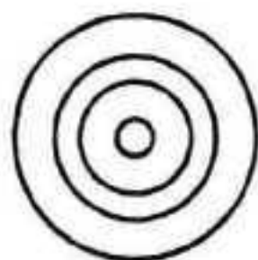
Warmth ether: spherical forms
