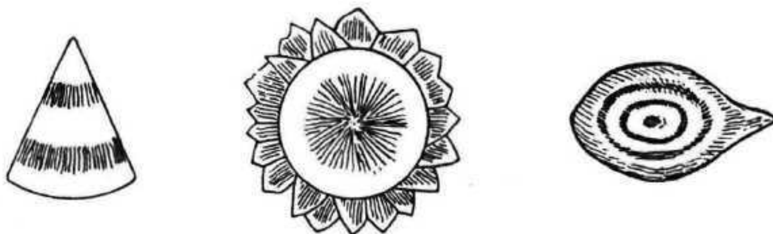
Hail stones (after Professor Trabert)
