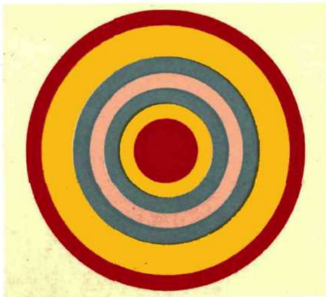
Earth with its Interior (represented as differentiated)
