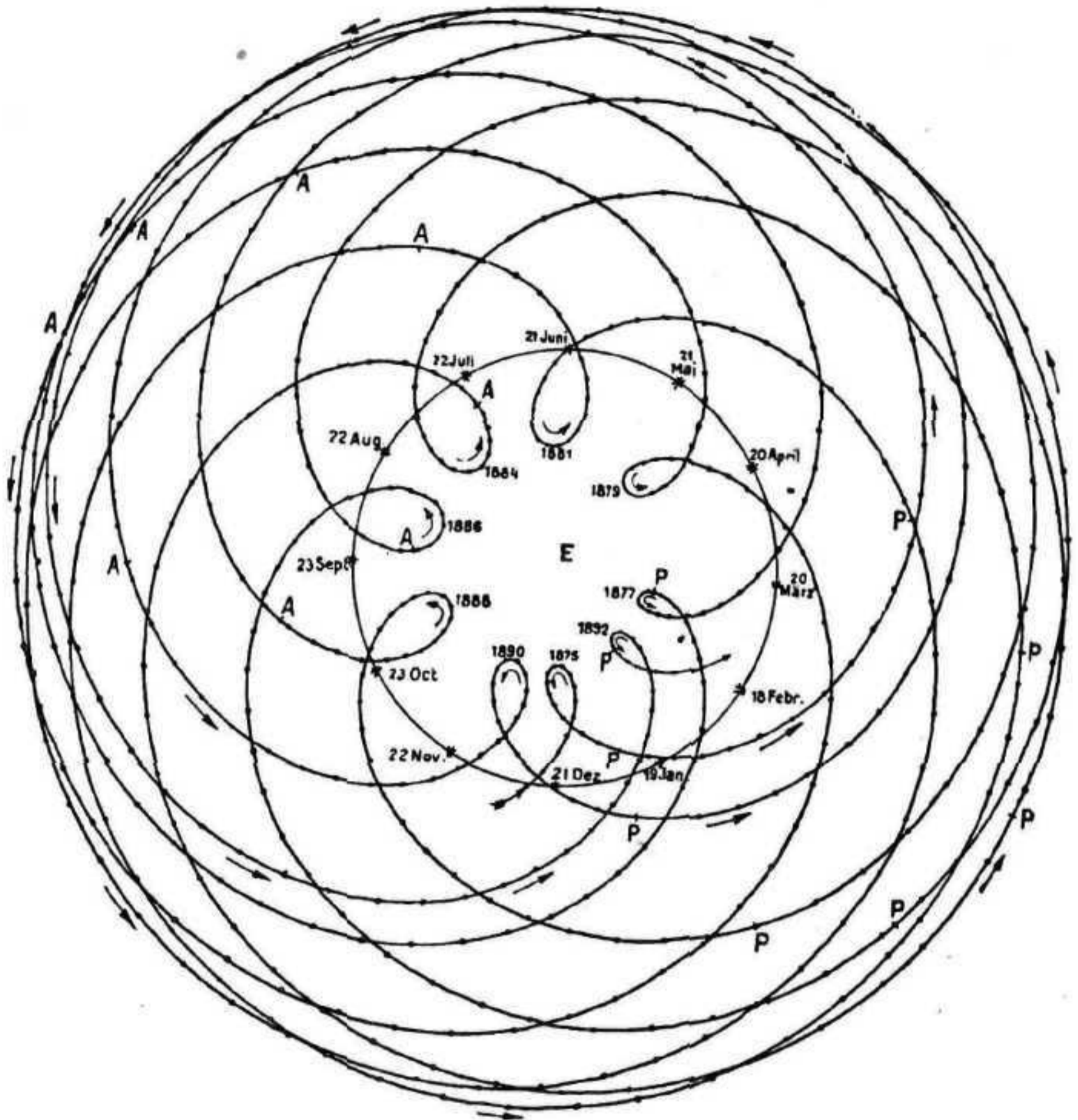
Epicyclic motion of Mars (after Plassmann).
