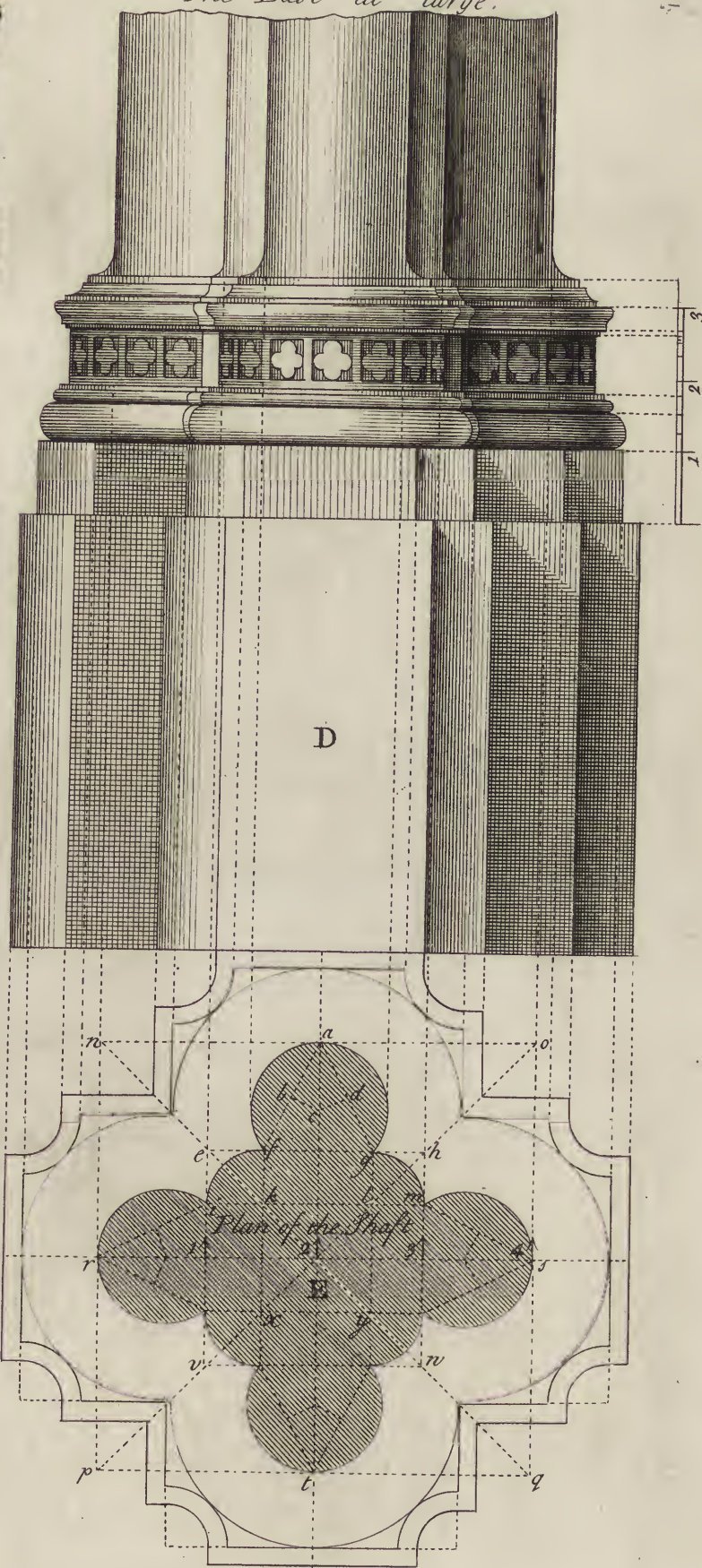
The Divisions of the Members in the Base at large.
