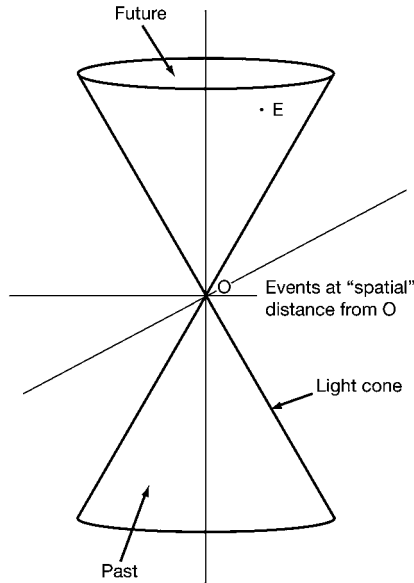
Figure 1.2. Light cones (after Anderson 1967, p. 154)
