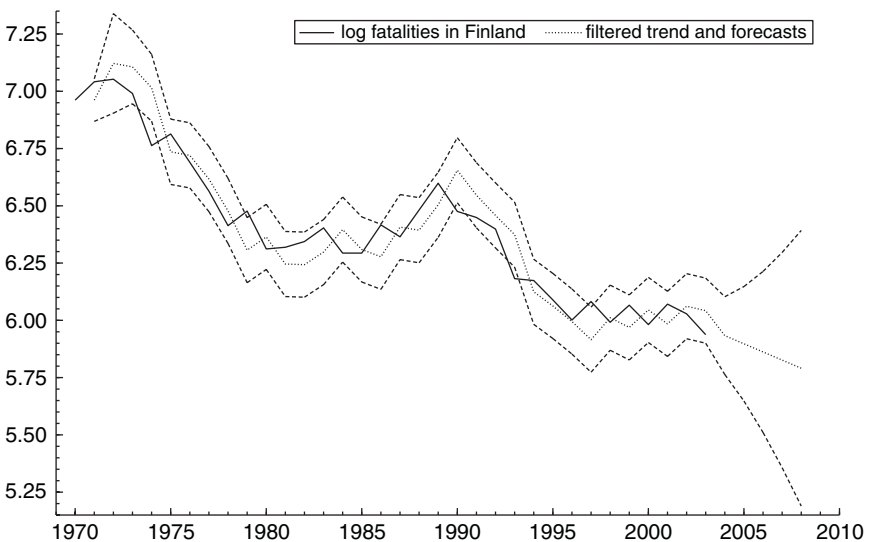
Figure 8.14. Filtered trend, and five-year forecasts for Finnish fatalities, including their 90% confidence limits.
