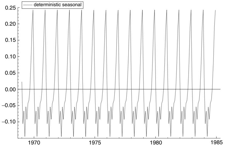
Figure 4.4. Deterministic seasonal.
