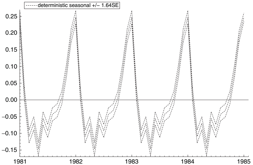
Figure 8.3. Deterministic seasonal and its 90% confidence interval for stochastic level and deterministic seasonal model applied to the log of UK drivers KSI.
