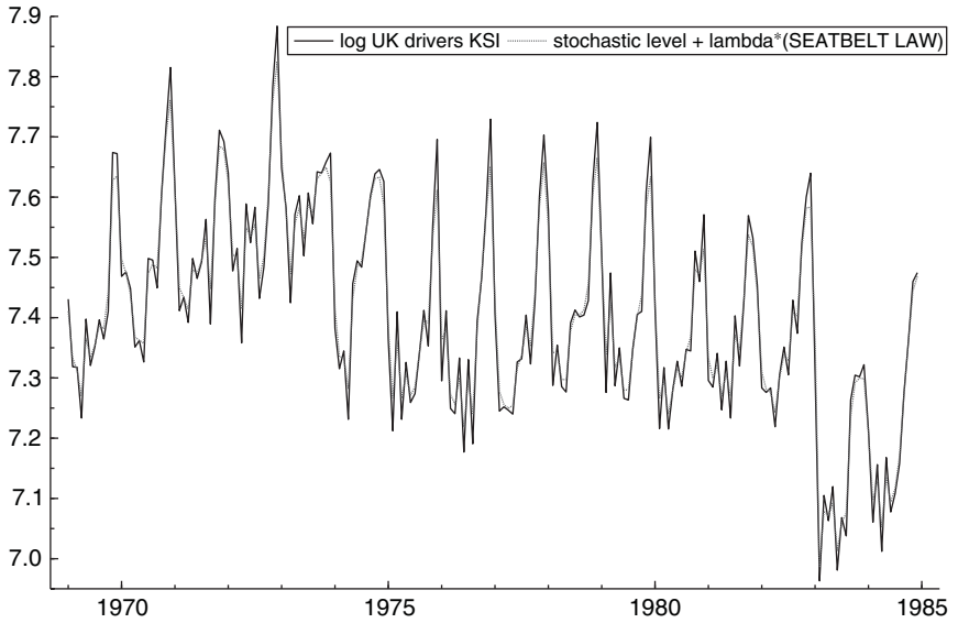
Figure 6.4. Stochastic level and intervention variable.
