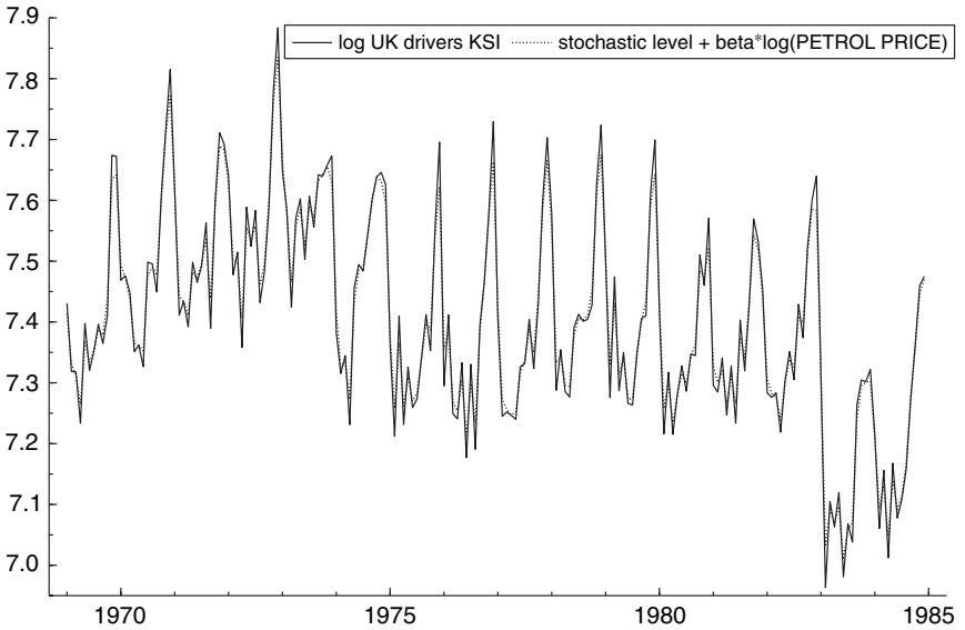
Figure 5.4. Stochastic level and deterministic explanatory variable 'log petrol price'.
