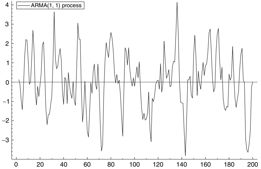
Figure 10.9. Realisation of an ARMA(1, 1) process with a_1 = \beta_1 = 0.5 .
