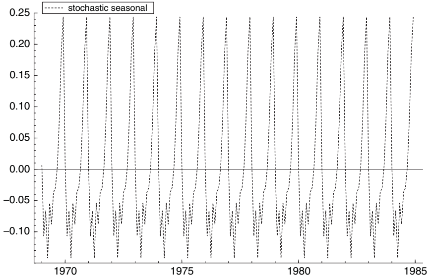
Figure 7.3. Stochastic seasonal.
