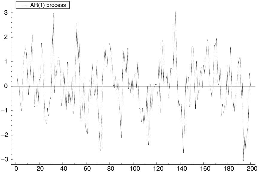
Figure 10.7. Realisation of an AR(1) process with \alpha_1 = 0.5 .
