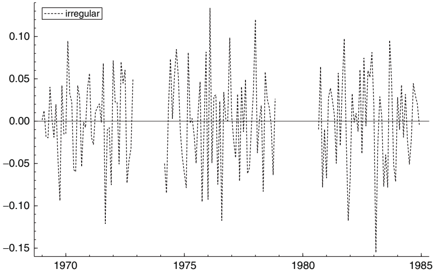
Figure 8.21. Irregular component.
