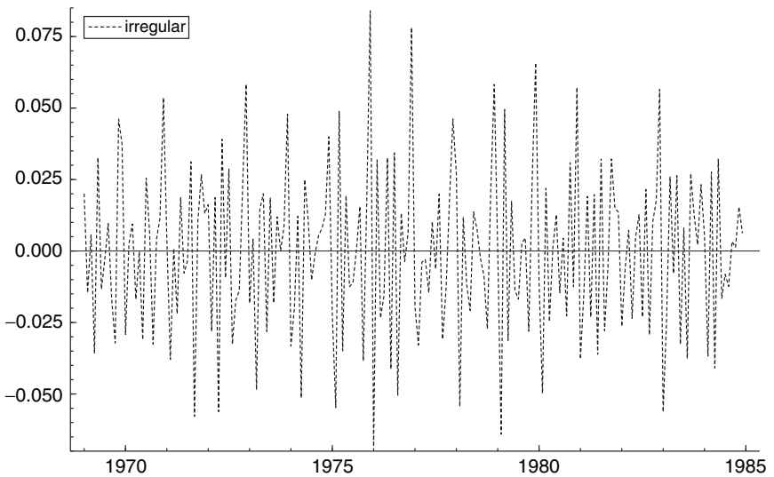
Figure 6.5. Irregular component for stochastic level model with intervention variable.
