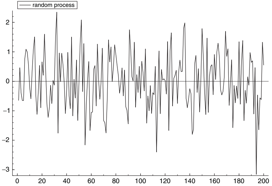
Figure 10.1. Realisation of a random process.
