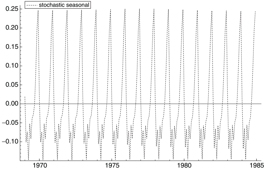
Figure 4.7. Stochastic seasonal.
