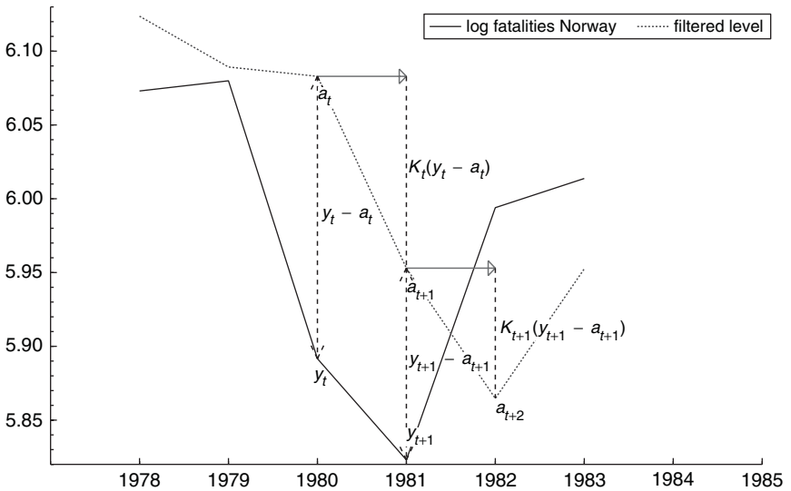
Figure 8.6. Illustration of computation of the filtered state for the local level model applied to Norwegian road traffic fatalities.
