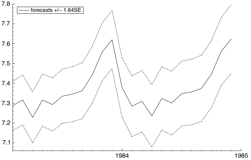
Figure 8.15. Forecasts for t = 170, \dots, 192 including their 90% confidence interval.
