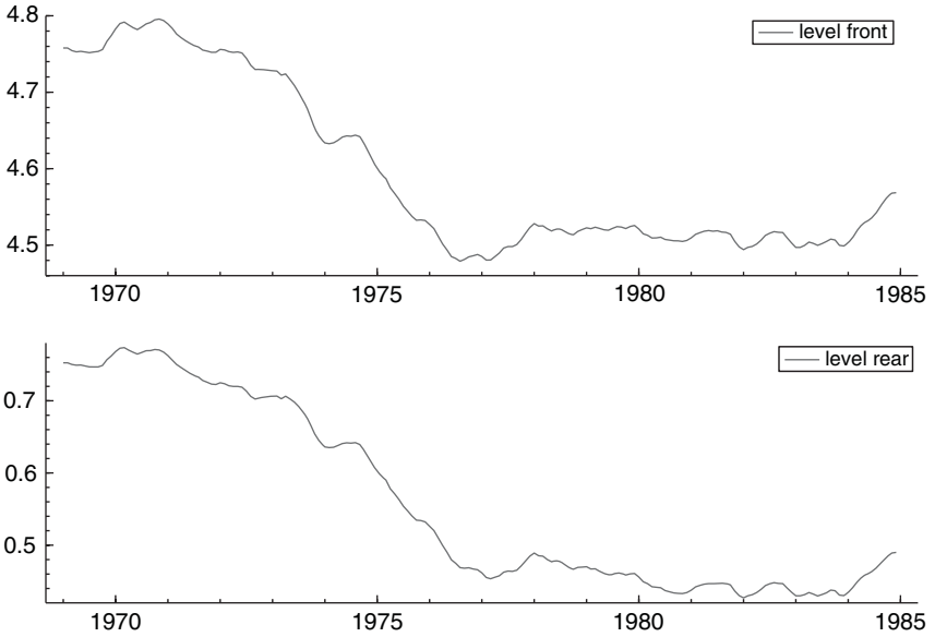
Figure 9.3. Levels of treatment and control series in the seemingly unrelated model.
