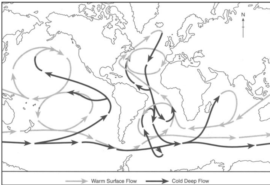
28. The deep circulation of the ocean, termed the oceanic conveyor belt
