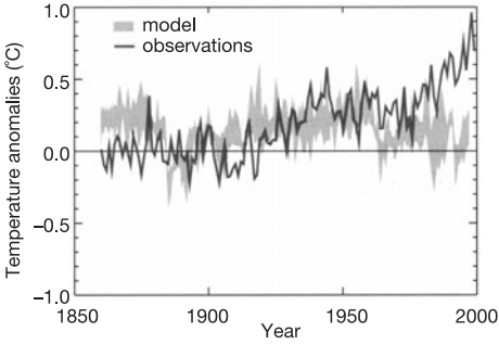
(b) Anthropogenic
