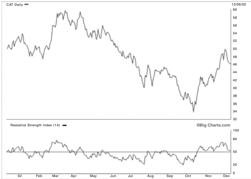
Figure 12-3 Relative strength indicator
