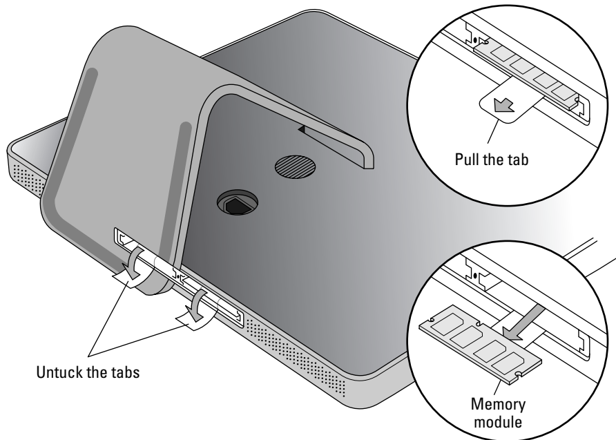
Figure 19-2: Remove a memory module like a pro.
