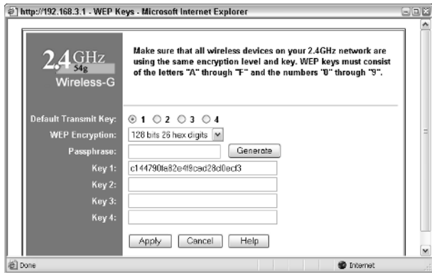
• Figure 46-5: The Linksys WRT54G’s WEP encryption key goes in a specific box. Other routers are similar.
