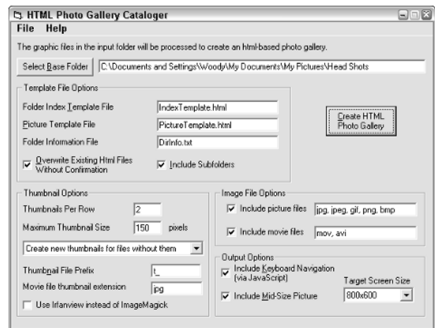
• Figure 43-5: HTML Photo Gallery Cataloger creates a page of thumbnails and turns a bunch of pictures into interlocked Web pages.
