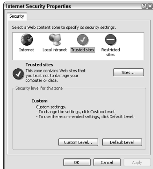
• Figure 23-22: Control the security of each zone and assign sites to zones in this dialog box.
