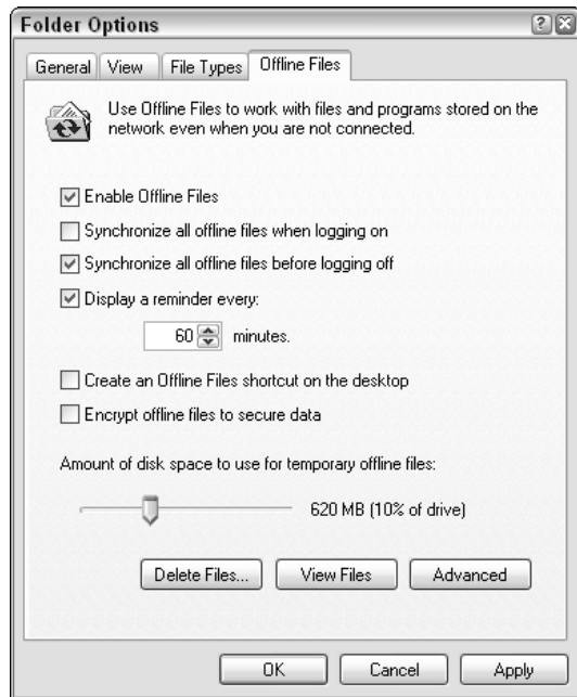
• Figure 1-5: Offline Files synchronize themselves automatically.
