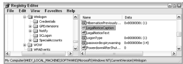
• Figure 8-4: Windows Registry entries that control the pre-logout screen.
