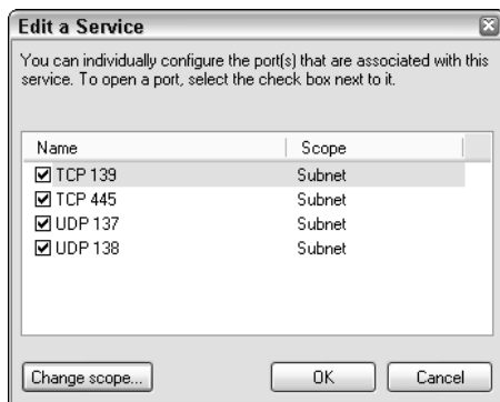
• Figure 50-5: File and Printer Sharing uses a set of four ports.
