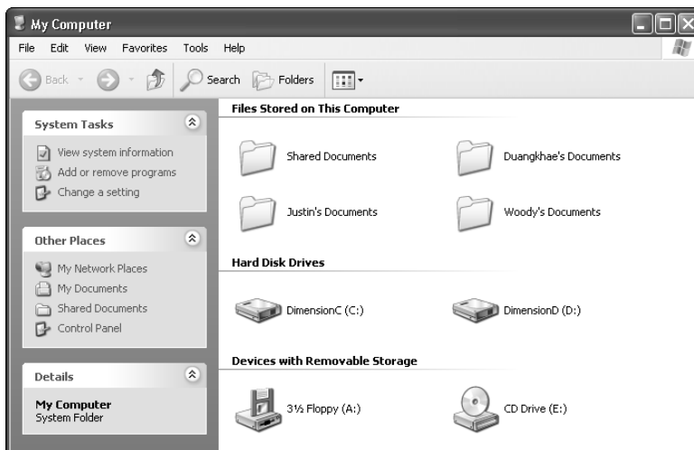
Figure 3-9: My Computer.
