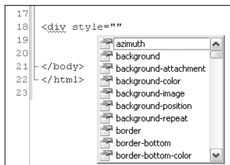
Figure 5-19: IntelliSense menu.
