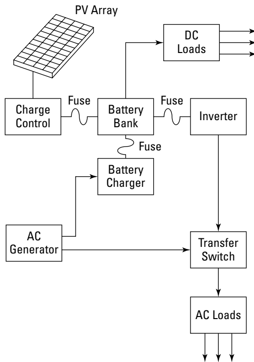
Figure 18-1: An off-grid, standalone, solar, PV power system.
