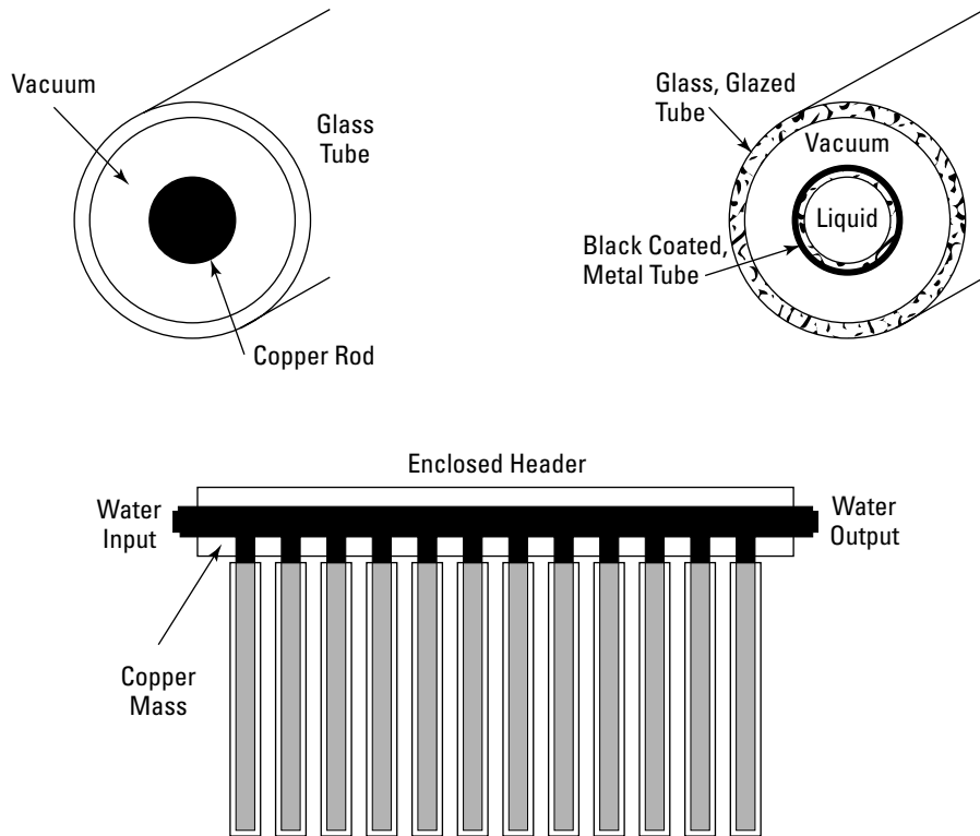
Figure 10-4: Construction details of an evacuated tube collector.
