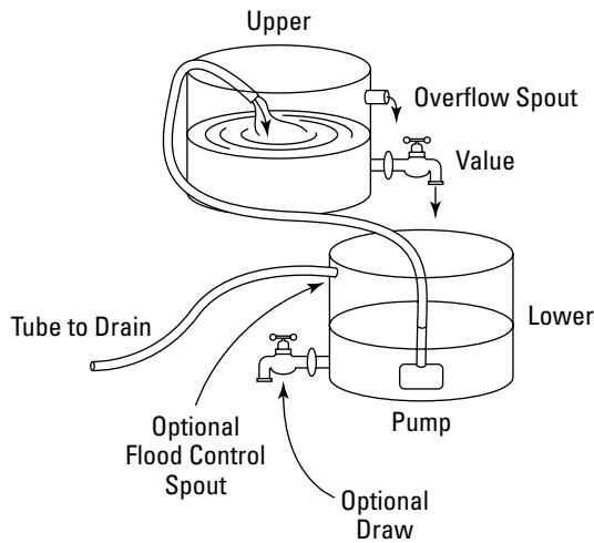
Figure 8-1: A wooden barrel solar fountain.
