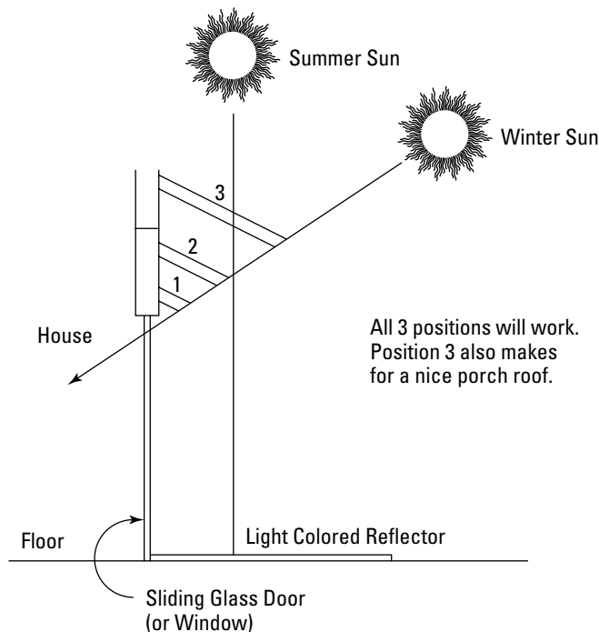
Figure 8-3: Overhangs control sunshine over the seasons.
