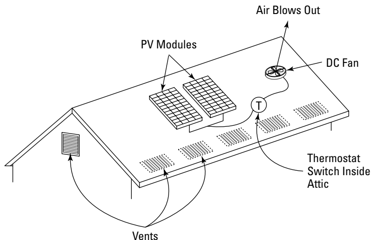
Figure 13-7: A PV module powers the attic vent fan, allowing hot air to escape when the sun shines its brightest.
