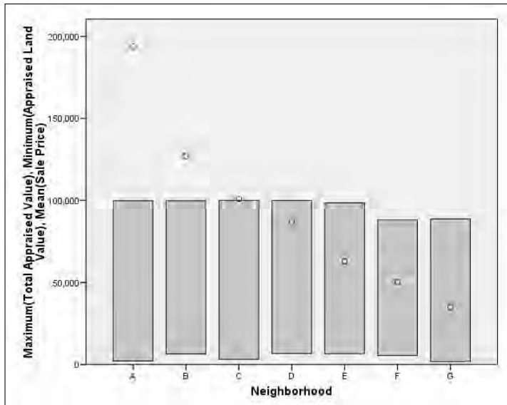
Figure 11-12: A high-low graph displaying a variable that curves out of its high and low limits.
