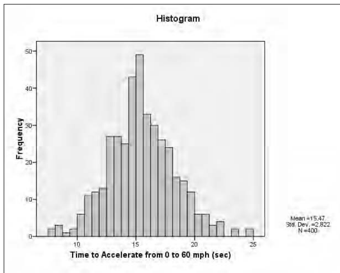
Figure 16-12: A histogram of acceleration rates.
