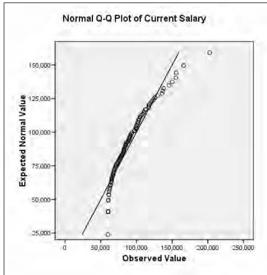
Figure 16-7: A q-q plot produced by the P PLOT command.
