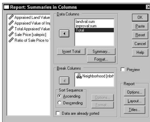
Figure 13-12: The variables that will appear in the summaries in columns report.
