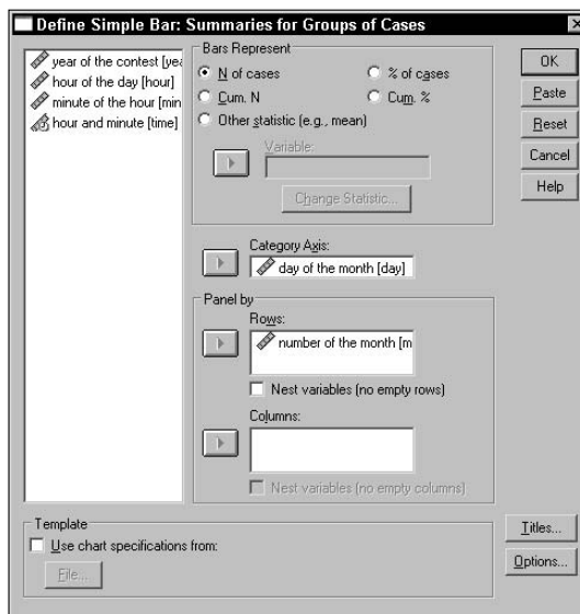
Figure 3-21: Selecting the data to include in the bar chart.
