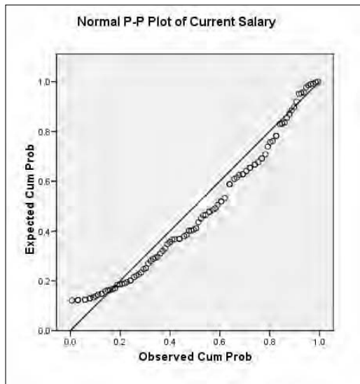
Figure 16-8: A p-p plot produced by the P PLOT command.
