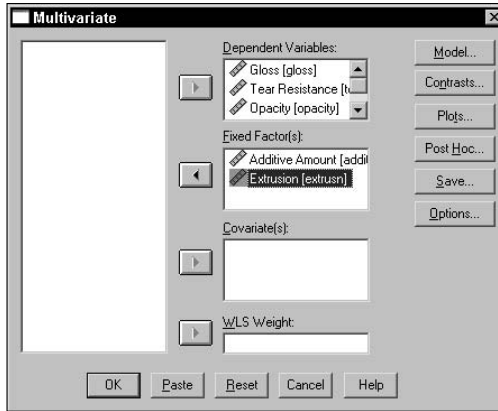
Figure 14-12: Three dependent variables are tested against two independent variables.
