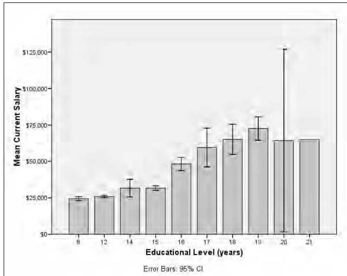
Figure 10-14: A bar chart with error bars showing the range containing 95 percent of all values.
