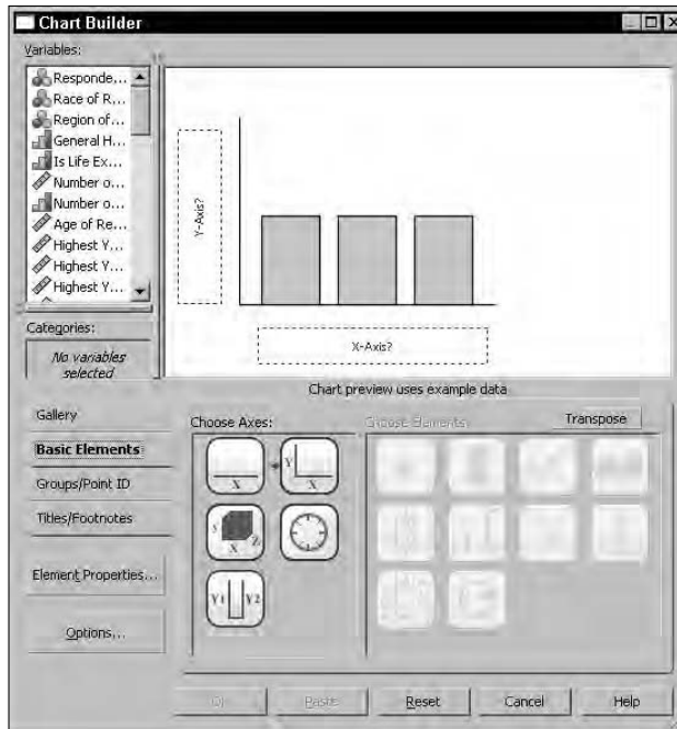
Figure 9-2: The appearance of the new bar chart is defined.
