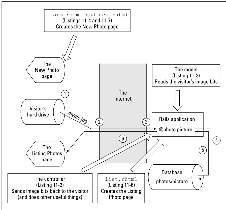
Figure 11-5: How code cooperates to create the photo album application.
