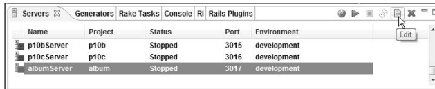
Figure 17-7: Finding the Servers view's Edit button.
