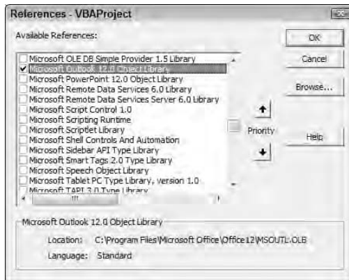
Figure 7-17: Adding an Outlook library reference to your application.
