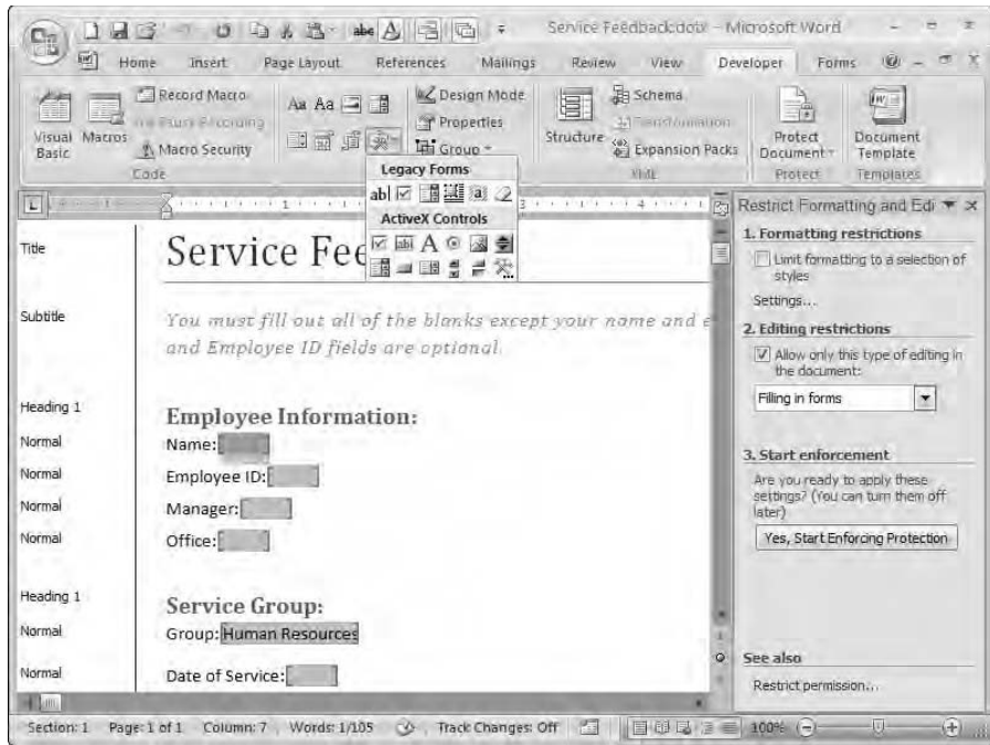
Figure 6-12: Choose the controls you want to use from the special Legacy Forms gallery.
