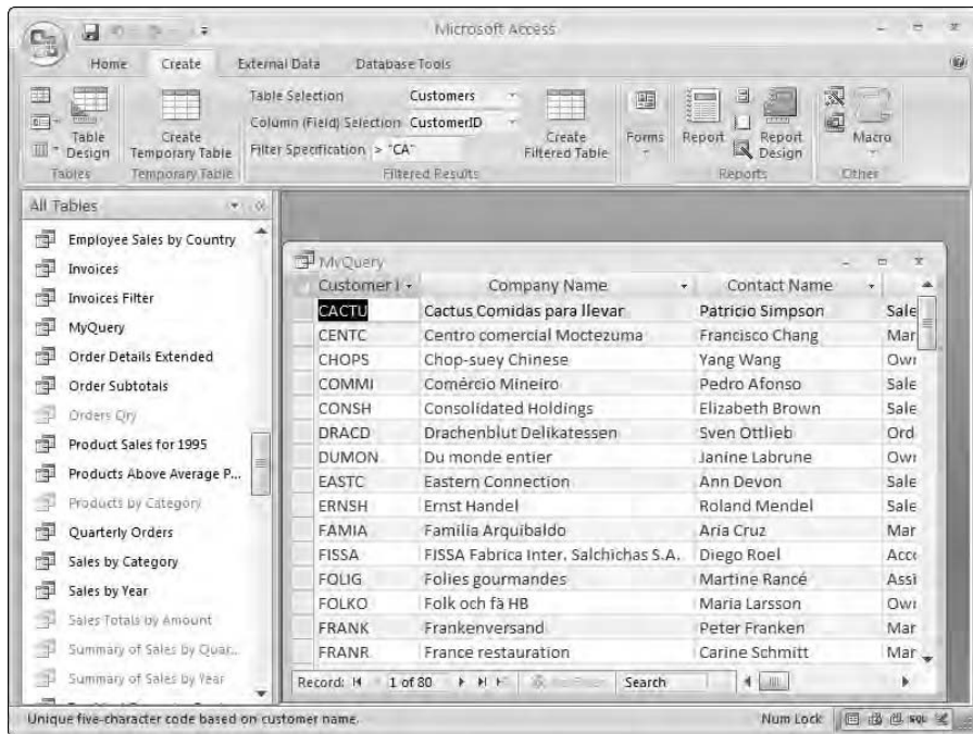
Figure 8-16: The new Create tab includes entries for temporary and filtered result tables.
