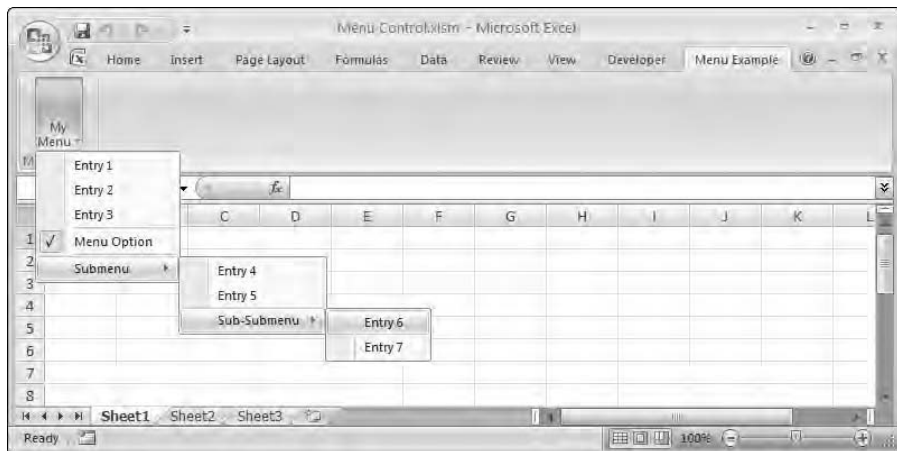
Figure 12-5: Create menus to mimic the menus you used in previous versions of Office.
