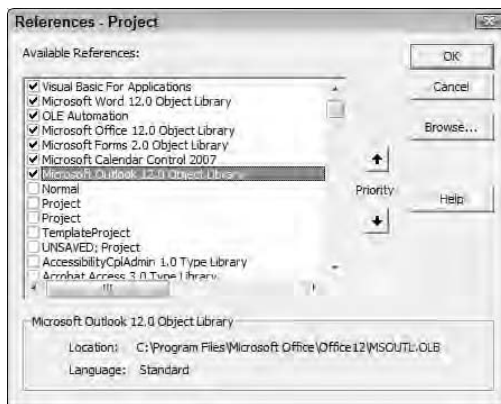
Figure 6-3: Add a reference to Outlook so your Word code can interact with it.
