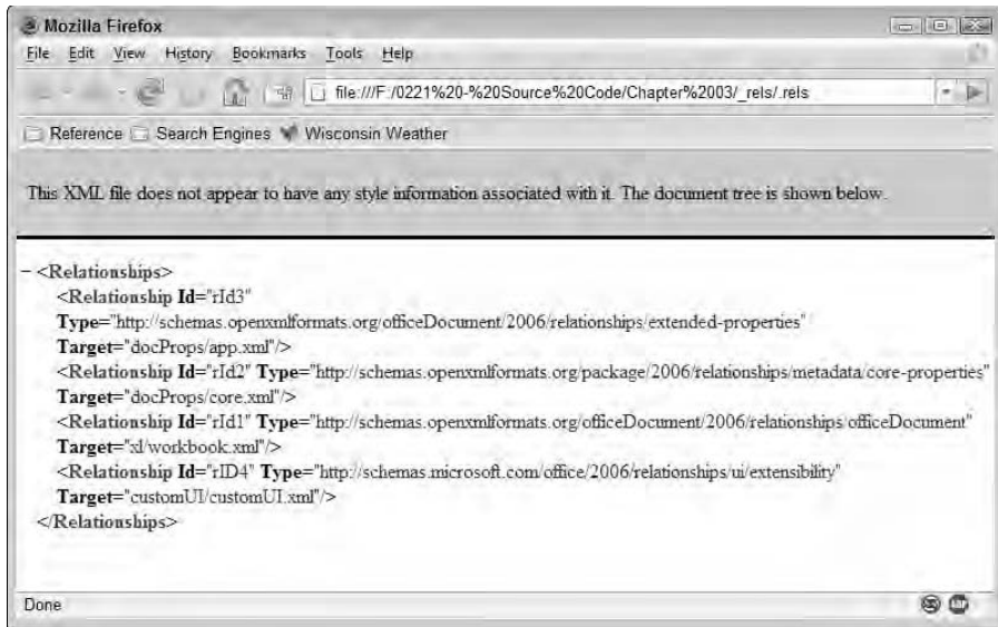
Figure 3-1: The .rels file contains one entry for each Excel relationship.
