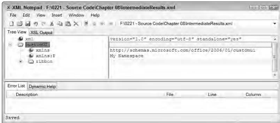
Figure 8-15: Create a custom namespace for your groups and controls.
