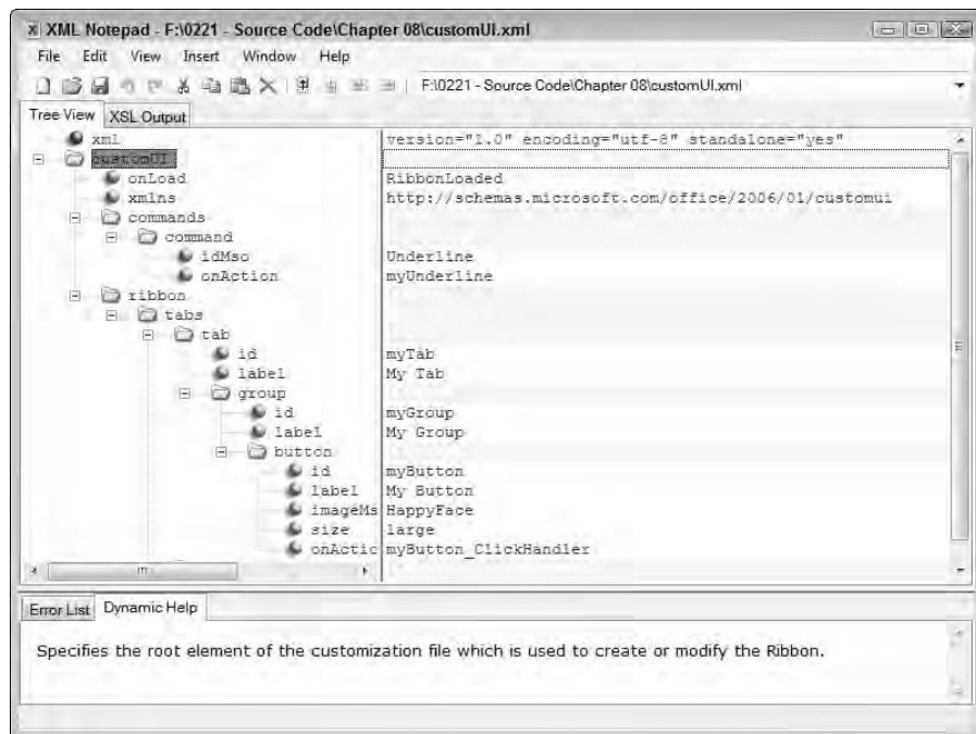
Figure 8-1: Use XML Notepad 2007 to perform edits of your Access XML files.
