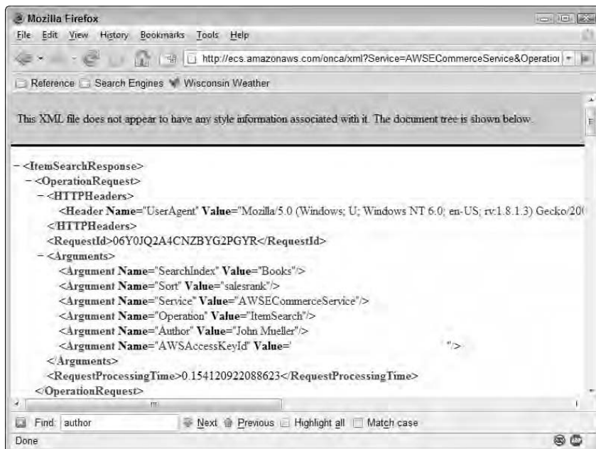
Figure 11-1: Experiment with AWS using a simple browser.
