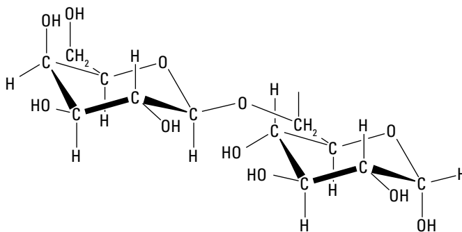
Figure 16-11: Structures of lactose and allolactose.
