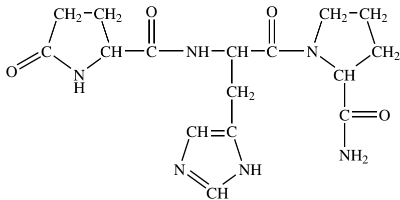
Thyrotropin-releasing factor
