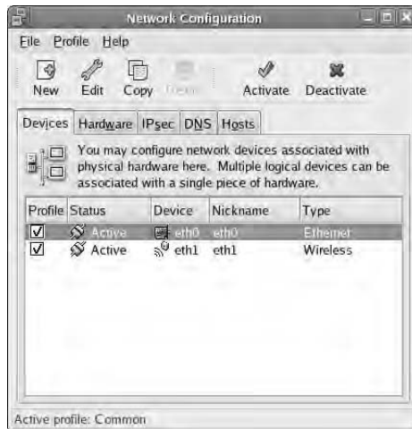
Figure 2-3: In Fedora Core, configure the Ethernet network with this network-configuration tool.
