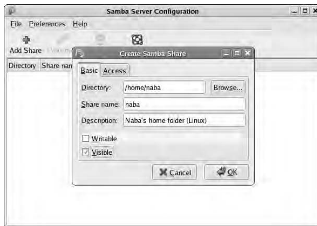
Figure 6-1: Adding a Samba share in Fedora Core.
