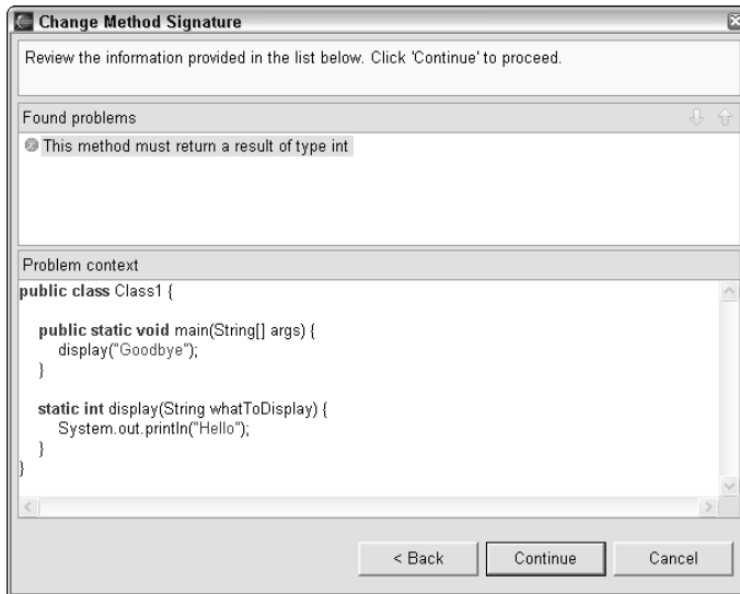
Figure 11-8: Excuse me. Eclipse says you have a problem.
