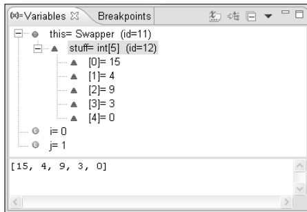
Figure 16-2: The Variables view (before executing stuff stuff [i] = stuff[j] ).
