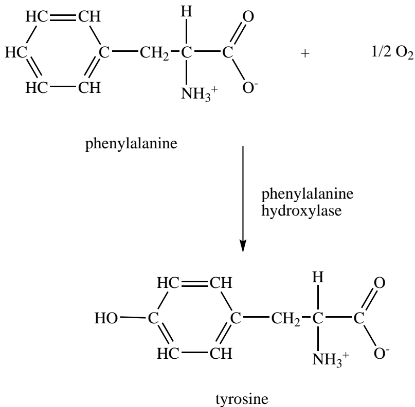
Figure 13-24: Synthesis of tyrosine.
