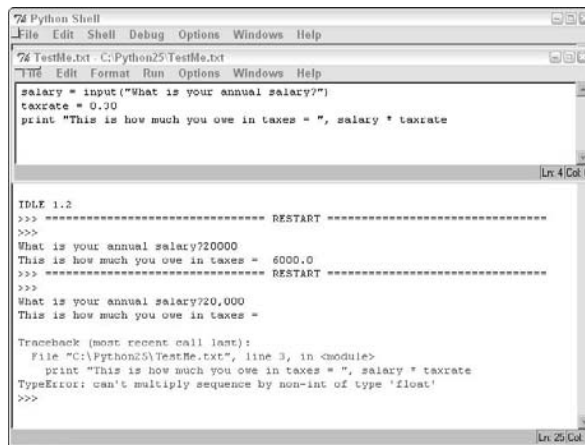
Figure 2-1: If a program tries to store the wrong type of data in a variable, the program stops running.
