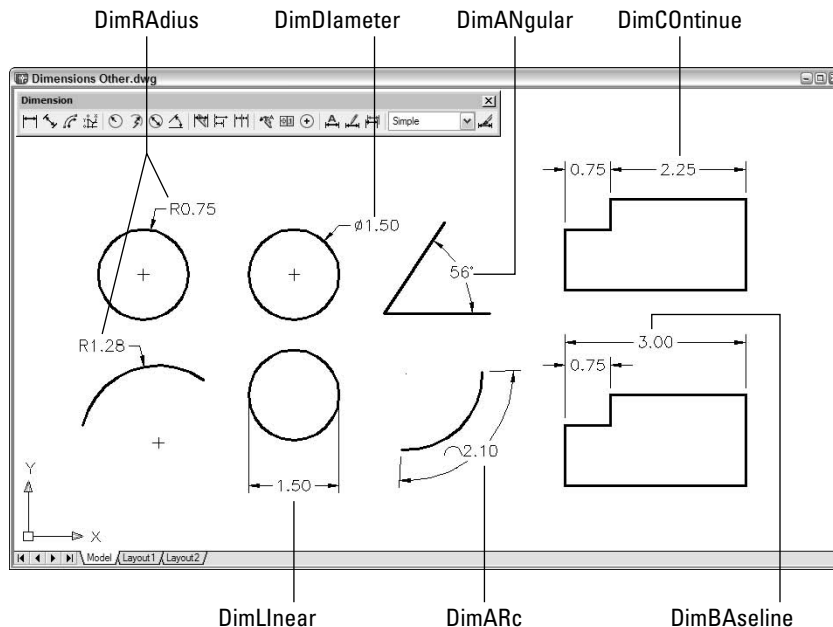
Figure 11-10: Examples of additional dimensioning commands.
