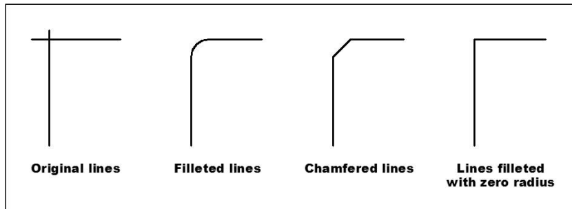
Figure 7-13: Cleaning up those corners with FILLET and CHAMFER.
