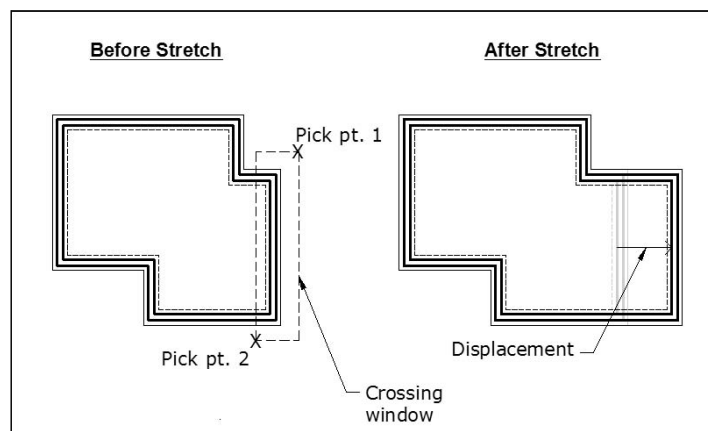
Figure 7-7: Use a crossing selection box to select objects for stretching.
