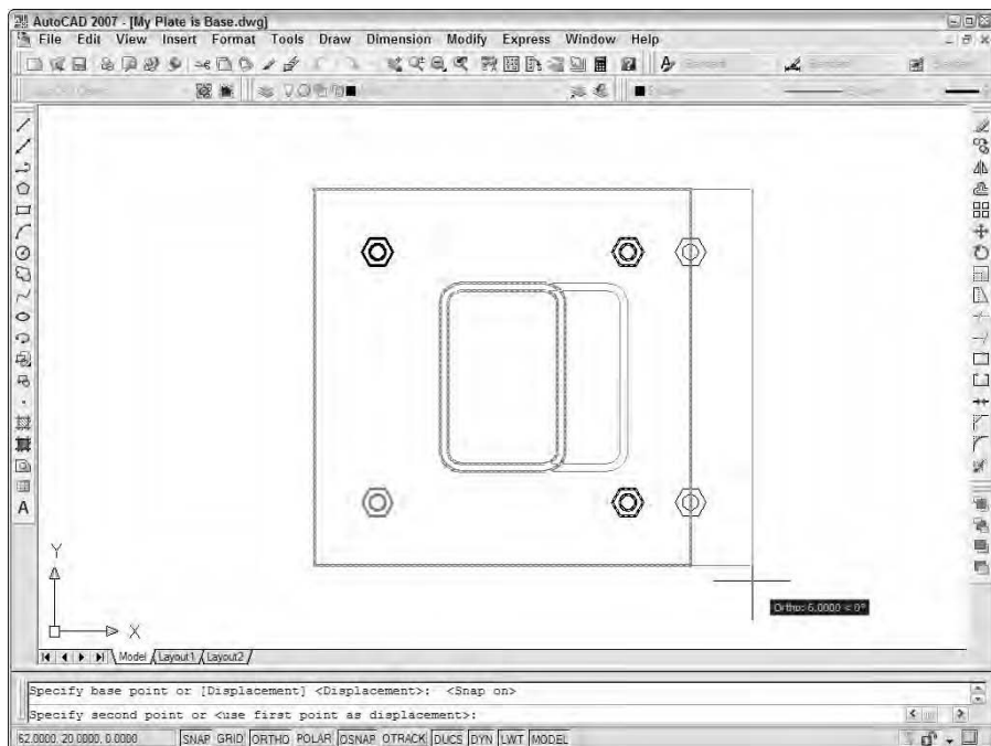
Figure 3-11: Stretching the base plate.
