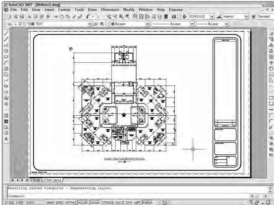
Figure 2-10: Freshly laid out in paper space.
