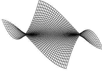
Fig. 5.3. The monkey saddle at (0, 0) is a degenerate critical point.
