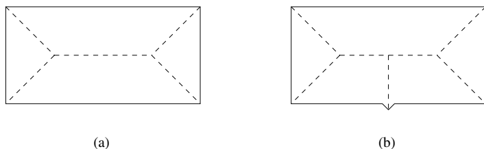
Fig. 13.10. The dashed medial axis of the solid polygon (a) is ill-conditioned as a small perturbation changes the resulting axis dramatically (b).
