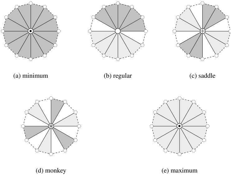
Fig. 6.6. Classifying vertices by their stars. The light-shaded lower wedges are connected by white triangles to the dark-shaded upper wedges. The dotted vertices and dashed edges on the boundary do not belong to the open star.
