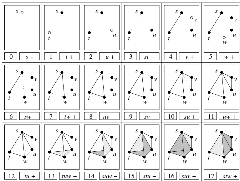
Fig. 7.2. A small filtration of a tetrahedron with a flap. The lightly shaded simplex is added at time i . The simplices are named and marked according to persistence.
