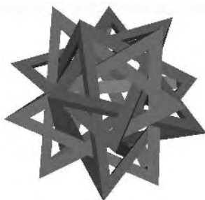
Fig. 6.15. The skeletons of 5 regular tetrahedra defined by the 20 vertices of the regular dodecahedron. The tetrahedra are linked pair-wise.
