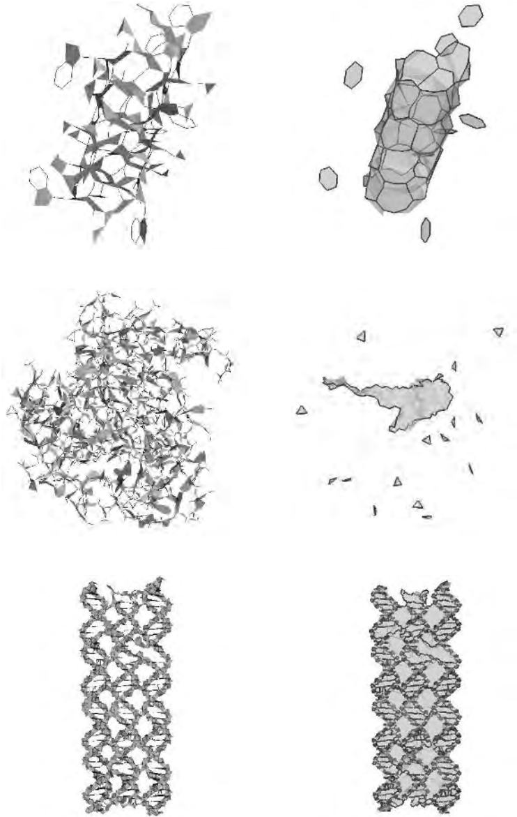
Fig. 10.8. Complex K^{1123} of the filtration for data set Igrm (top) has 1 component and 34 basis cycles. Complex K^{8168} of Ihck has 2 components and 17 cycles. Complex K^{90000} of TAO (bottom) has 1 component and 237 cycles. In each case, the spanning surfaces are rendered transparently.
