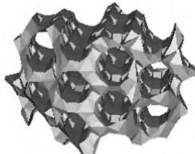
(e) K^{24811} of BOG
