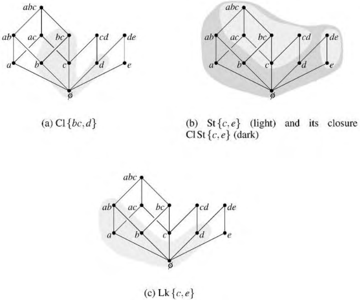
Fig. 2.12. Closure, star, and link of simplices.
