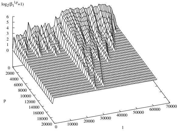
(a) Graph of \log_2(\beta_1^{l,p} + 1)
