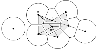
Fig. 2.16. Union of nine disks, convex decomposition using Voronoi regions, and dual complex.
