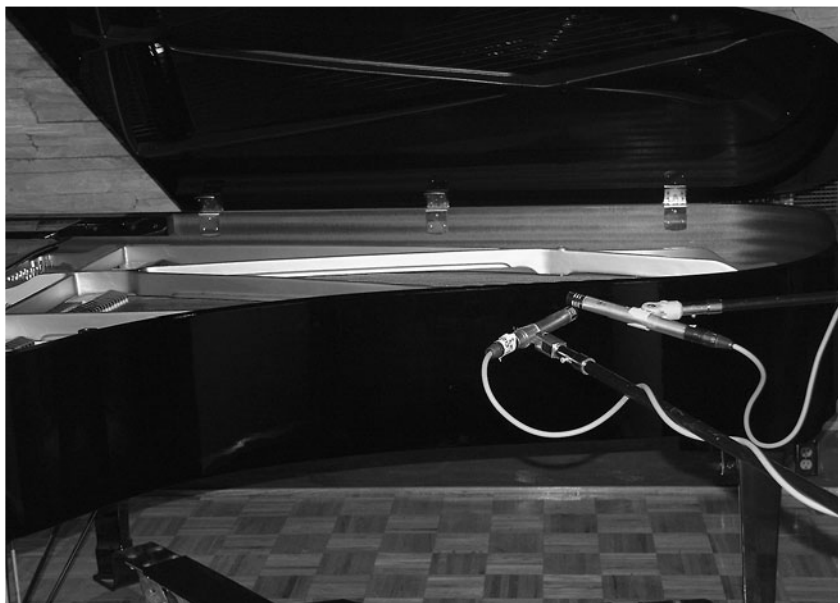
Figure 117 AKG 452s in X/Y Outside of Piano
