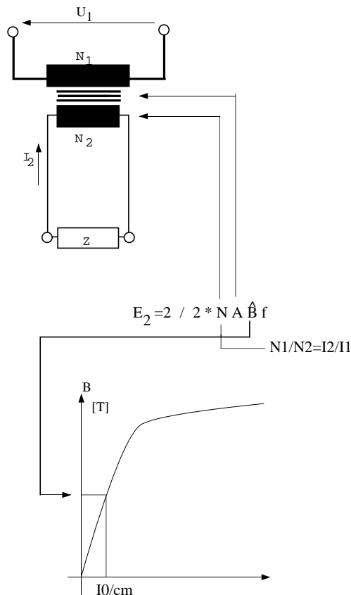
Figure 2. The factors influencing the voltage transformer output and magnetizing current.
