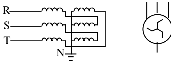
Figure 6. Z/0-connected earthing transformer.
