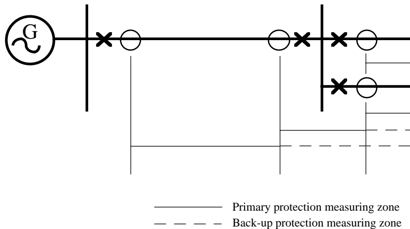
Figure 4. Primary and back-up protection zones
