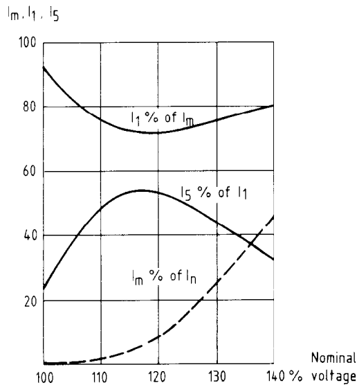
Figure 3. Magnetizing current at Overexcitation where “ I_1 ” is the fundamental frequency current, “ I_5 ” is the fifth harmonic current, “ I_m ” is the total magnetizing current and “ I_n ” is the nominal current.
