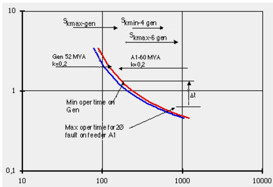
Figure 25. The selectivity plan shows that selectivity is achieved with similar settings due to the differences in fault currents.
