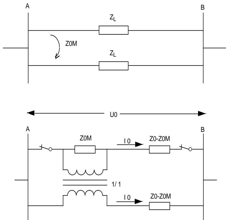
Figure 15. Influence of mutual impedance, at parallel lines, at the same tower.
