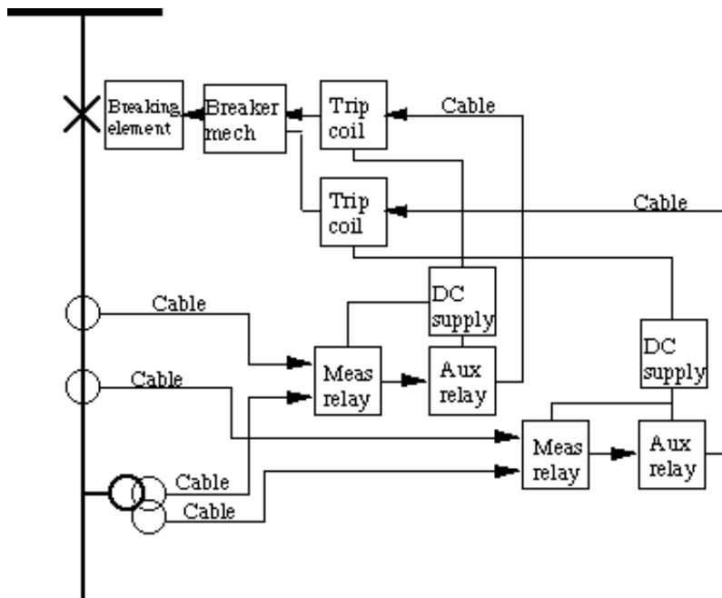
Figure 6. The fault clearance chain at redundant protection systems.
