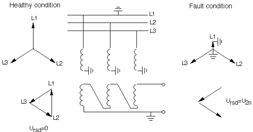
Figure 5. The principle for a open delta winding. Occurring voltages at an earth fault in a direct earthed system.
