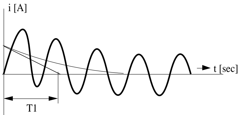
Figure 4. The primary fault current with a DC component.
