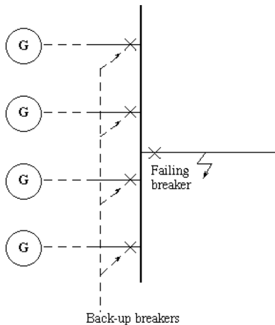
Figure 7. The principle of a breaker failure protection.
