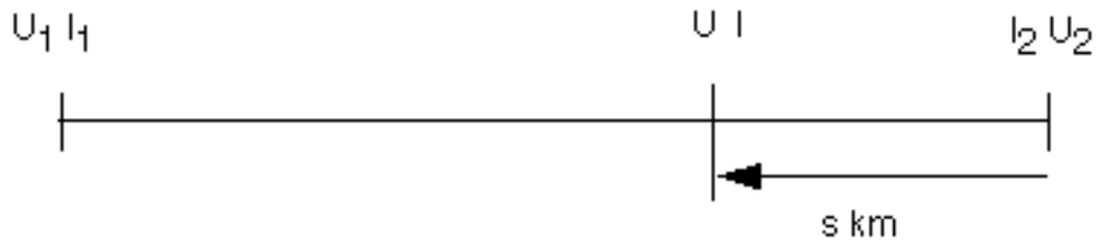
Figure 2. Voltage distribution along a line.
