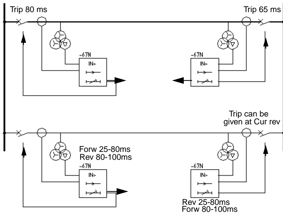
Figure 9. The current reversal problem at parallel lines.
