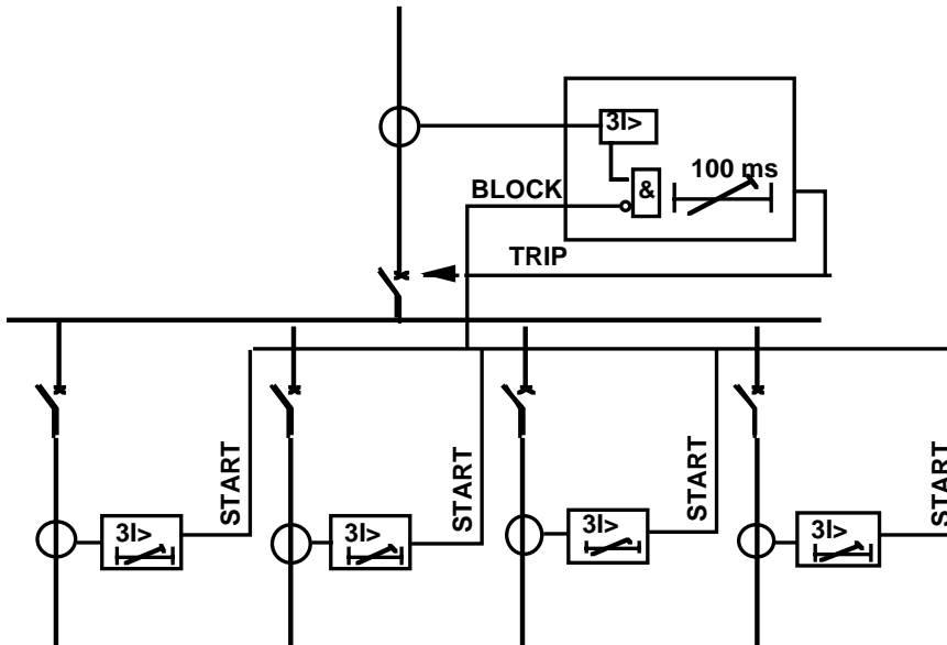
Figure 6. Blockable Overcurrent protection.
