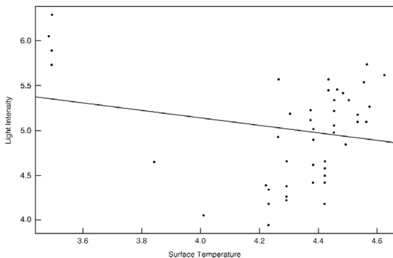
Figure 3.9 Surface temperature and light intensity of 47 stars.
