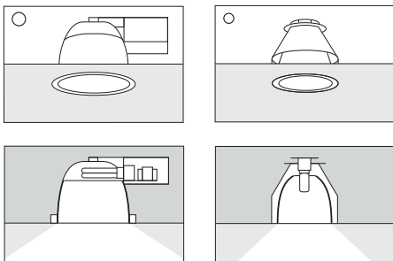
Recessed downlight for halogen lamps.
