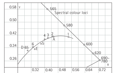
Section of the chromaticity diagram with the curve relating to the Planckian radiator and the colour loci of standard illuminants A (incandescent light) and D 65 (daylight) plus the colour loci of typical light sources: candle-light (1), incandescent lamp (2), halogen lamp (3), fluorescent lamps in ww (4), nw (5) and dw (6).
