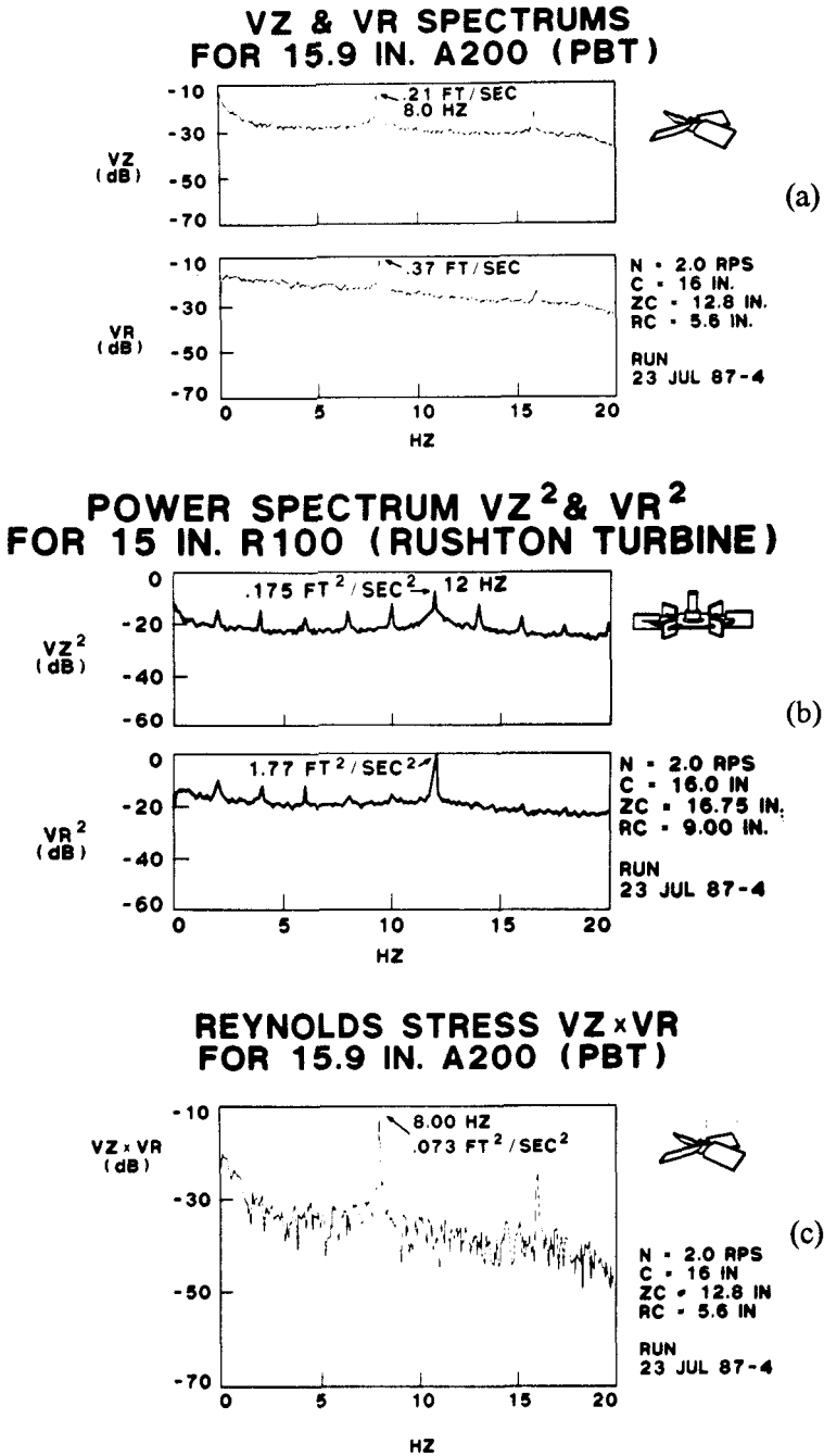
Figure 24. Typical spectrum analysis of the velocity as a function of (a) velocity frequency fluctuation, (b) the frequency of the fluctuations using the square of the velocity to give the energy dissipation, and (c) the product of two orthogonal velocities versus the frequency of the fluctuations. The product of two orthogonal velocities is related to the momentum in the fluid stream.
