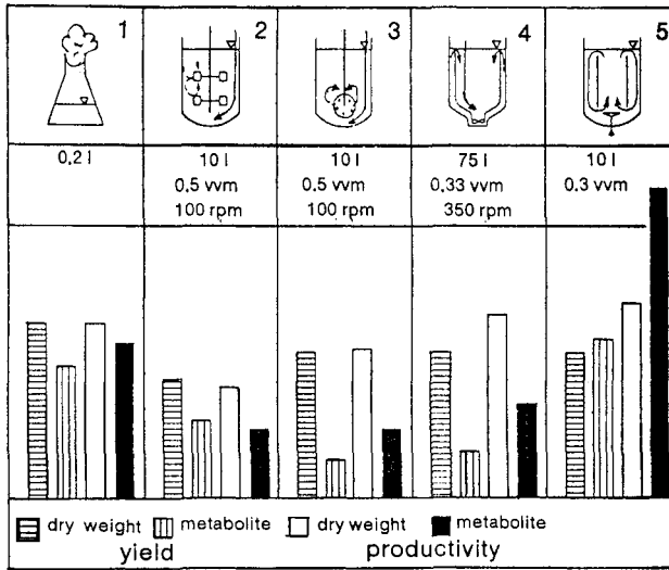
Figure 19. Comparison of yield and productivity for cell mass and anthraquinones in various bioreactor systems. (1) Shake Flask. (2) Flat Blade Turbine. (3) Perforated Disk Impeller. (4) Draft Tube Bioreactor with Kaplan Turbine. (5) Air-lift Bioreactor.
