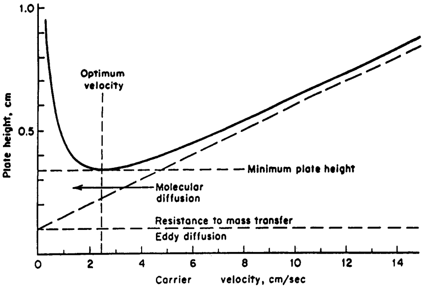
Figure 9. Relationship between late height and velocity of the mobile phase. [49]
