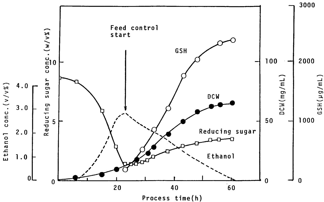
Figure 8. Trends of glutathione, reducing sugar, dry cell weight (DCW) and ethanol concentration in the broth during the glutathione fermentation in 120-kl fermenter using the feed-forward/feedback control system.
