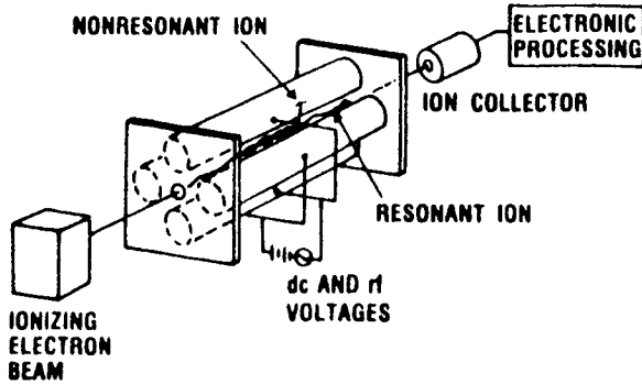
Figure 4. Quadrupole principle.
