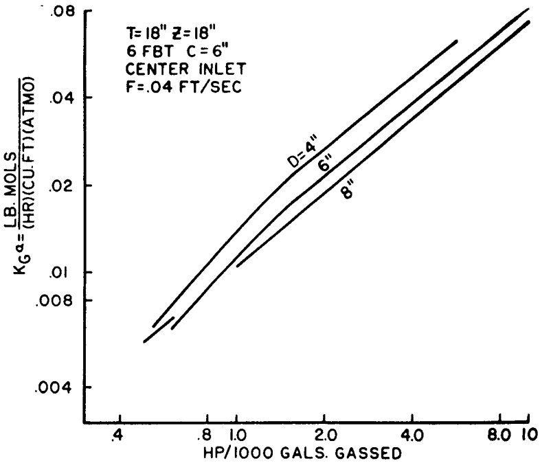
Figure 31. Effect of horsepower and impeller diameter on mass transfer coefficient at 0.04 \text{ ft/sec} gas velocity.
