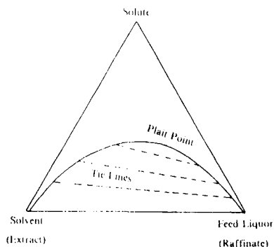
Figure 5. Ternary plot of distribution data.
