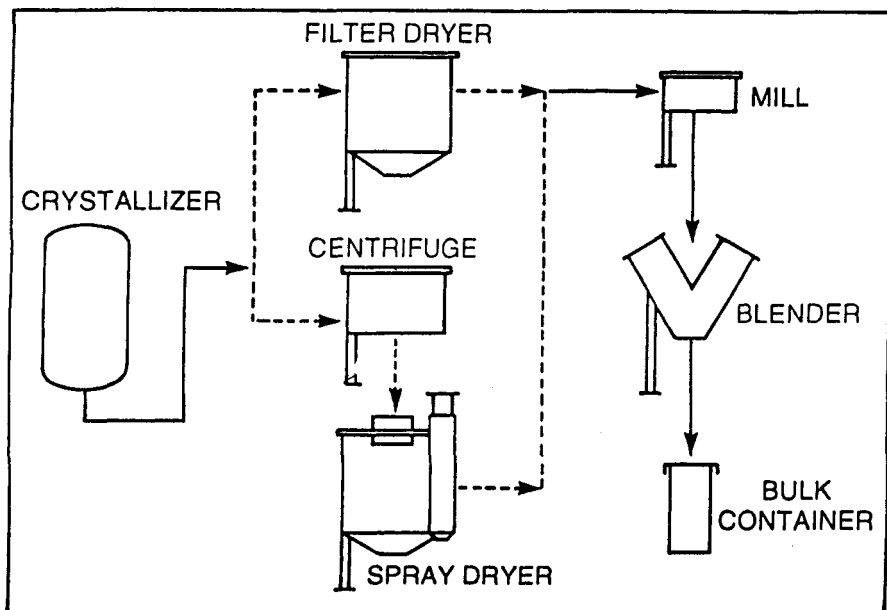
Figure 2. Typical isolation process for a filter/dryer or spray dryer
