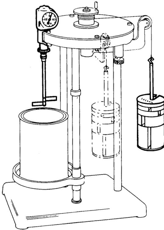
Figure 40. Schematic illustrating Stormer viscosimeter.
