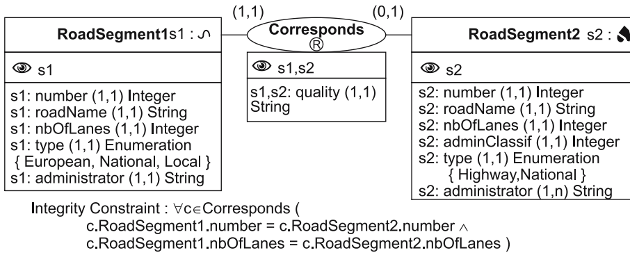
Modeling and Multiple Perceptions, Figure 15 The RoadSegment type (from Fig. 14) split into two monorepresentation object types and an interrepresentation relationship type
