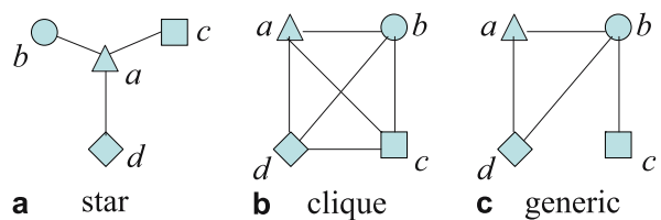
Co-location Patterns, Algorithms, Figure 1 Three pattern representations
