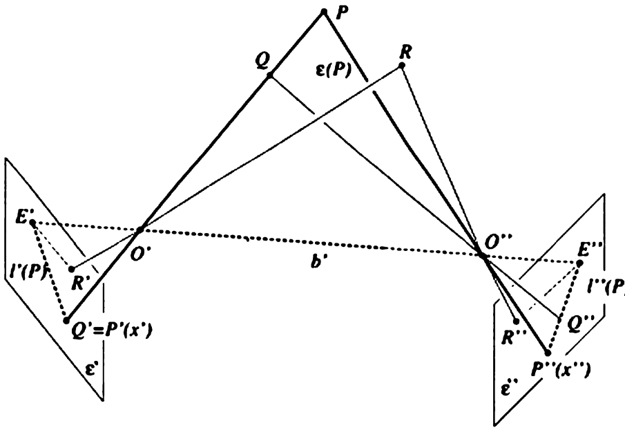
Photogrammetric Methods, Figure 3 Elements of the epipolar geometry: epipolar plane \epsilon(P) through O'O''P , with the epipoles E' and E'' as images of the other projection center ( O' or O'' ), the epipolar lines l'(P) and l''(P) which are the intersections of the epipolar plane \epsilon(P) and the image planes \epsilon' and \epsilon'' . The epipolar planes build a pencil of planes with the base line b' = O'O'' as axis, e.g., induced by a different point R . Therefore the epipolar lines also build a pencil of lines with the epipoles as carrier. Observe, P' does not allow inference of where P sits on the projecting line. Point Q , also mapping to P' , however, has a different image Q'' inducing the epipolar line l''(P) = (E'' Q'' P'') in the other image [1]
