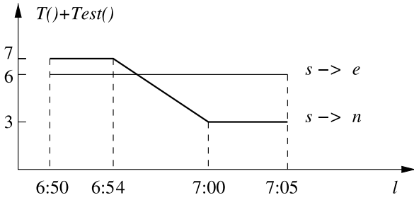
Fastest-Path Computation, Figure 2 Comparison of the functions T(l) + T_{est}(l) associated with paths s \rightarrow e and s \rightarrow n
