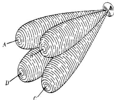
Figure F12 Beams formed with four-horn feed (from Rhodes, 1980, p. 70).
