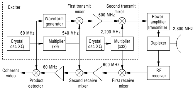
Figure E21 Coherent-radar exciter (after Fink, 1982, Fig. 25.82, p. 25.72).
