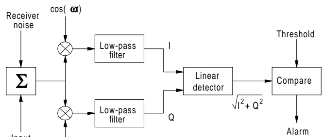
Figure D21 I/Q detection (after Blake, 1980,
