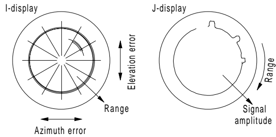
Figure D50 G- and H-displays.
