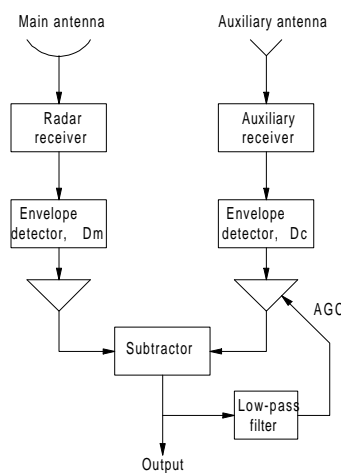
Figure C7 Noncoherent (video) sidelobe canceler (after Fielding, et al., 1977).
