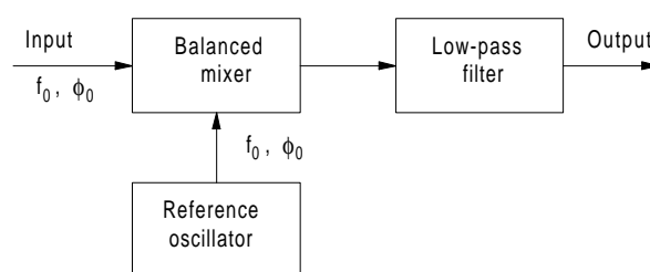
Figure D29 Basic configuration of a coherent detector (after Skolnik, 1980, Fig. 10.4, p. 385).
