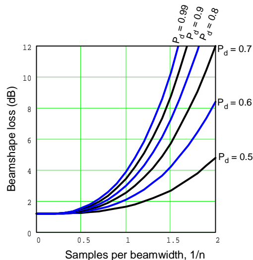
Figure L20 Beamshape loss for a steady target as a function of the beam motion between pulses or scan lines.
