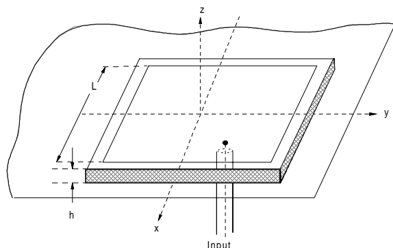
Figure A69 Microstrip antenna.
