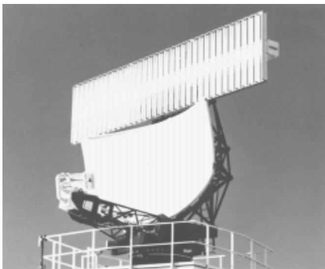
Figure A53 Coscant-squared antenna for ASR10SS radar.
