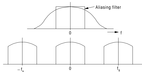
Figure A22 Antialiasing filter (after Currie, 1989, Fig. 6.9, p. 185).
