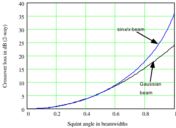
Figure A16 Conical-scan crossover loss (after Barton, 1969, Fig. 2.10, p. 37).
