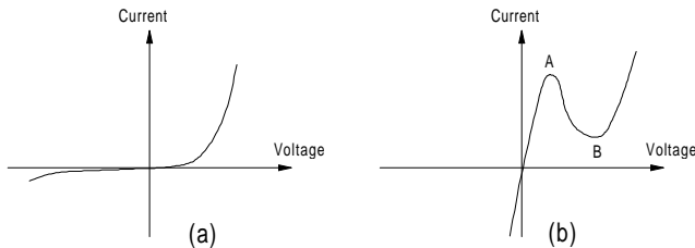
Figure D35 Voltage-ampere characteristic of (a) conventional and (b) tunnel diodes (after Leonov, 1988, Fig. 2.15, p. 52).
