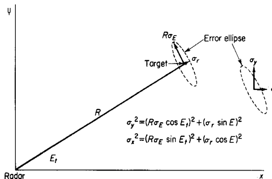
Figure U1 Target uncertainty ellipse (from Barton (1969), p. 241).
