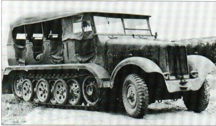
The Czech-built Praga SdKfz 6s featured longer track bogies than the Bussing-NAG models, and had different wings. They were powered
