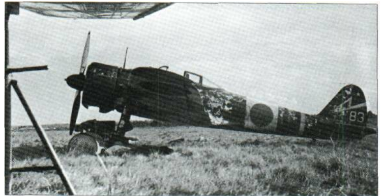
Right: A Ki-43-Ib of the 47th Independent Fighter Chutai at rest on a Japanese airfield. After service in all theatres throughout the war, the Ki-43 soldiered on against the Allies, but many were expended in kamikaze attacks.
