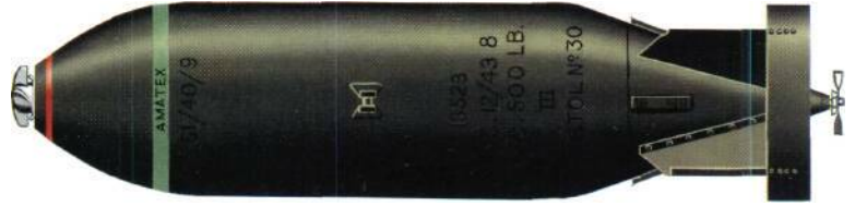
Right: The 227-kg (500-lb) MC, MkIII HE bomb was much more effective than the earlier 500-lb GP bomb, due to a higher filling-to-overall weight ratio. The cropped annular vane permitted four of these bombs to be carried by the Mosquito bomber. It did not affect stability.
