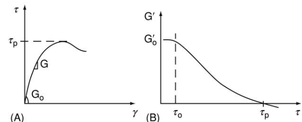
Figure 12 Stiffness and shear modulus.
