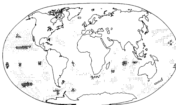
Figure 4 Distribution of manganese nodules in the oceans (updated from Cronan, 1980 after various sources.) : : : , Areas of nodule coverage; ▣▣▣, areas where nodules are locally abundant.
