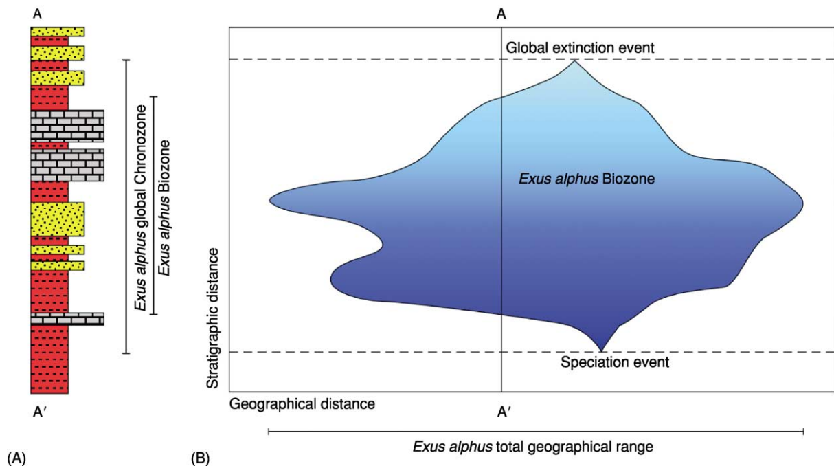
Figure 8 Relation between the (hypothetical) Exus alphus Biozone and its corresponding chronozone. (A) Zone expression at the level of a local stratigraphic sequence A–A'. (B) Two-dimensional slice through the Exus alphus Biozone containing the A–A' sequence. Note that the rock-stratigraphic expression of the local biozone (which also represents a local chronozone) underestimates the extent of the global chronozone based on the interval between the species' speciation and global extinction horizons. See text for discussion.
