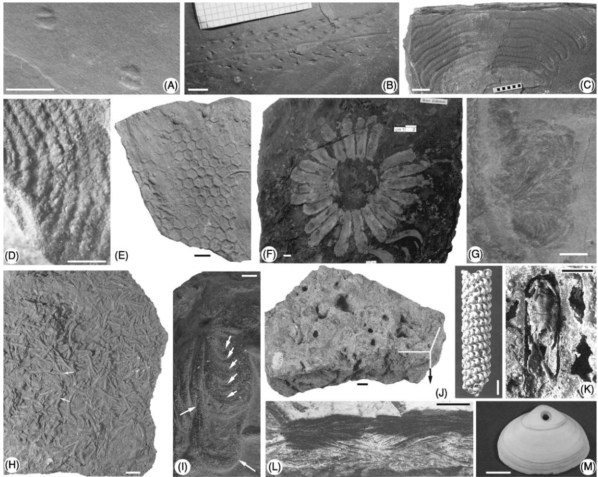
Figure 7 Variation in behaviour represented by trace fossils. (A) The cubichnion, Rusophycus . (B) An arthropod-produced repichnion. (C) The pascichnion, Nereites , exhibiting strophotactic and thigmotactic behaviour. (D) The consistent sense of braiding between successive burrows indicates thigmotactic behaviour achieved by spiralling alone. (E) The agrichnion, Paleodictyon . (F) Fodinichnion comprising unbranched shafts radiating parallel to bedding from a central area. (G) Fodinichnion comprising a series of lobate spreiten. (H) High-density, monospecific occurrence of the fodinichnion, Chondrites ; each burrow system comprises a series of branching shafts (at arrows) fanning outwards and downwards from a central shaft. (I) Protrusive spreite (short arrows) contained inside a U-shaped burrow (long arrows). (J) Oblique view of block of shallow marine oolitic limestone that was later bored and encrusted during emplacement of a hardground community. (K) External view and rare example of a pupa preserved inside the case constructed by a caddis fly larva. From Huguency M, Tachet H, and Escuillié F Caddisfly Pupae from the Miocene industrial Limestone of saint-Gerand-le-Puy, France (1990) Palaeontology 33: 495–502, Plate 1, Figures 3 and 4. (L) Bioglyph on the internal surface of a burrow excavated in semilithified sediments. Image courtesy of Richard Bromley, Copenhagen. (M) Praedichnion: a hole drilled by a gastropod through the shell of a bivalve. Scale bars, 5 mm.
