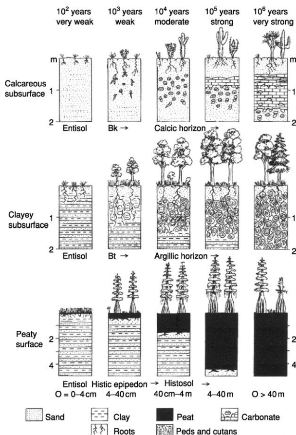
Figure 1 Soil development stages involving progressive calcification (top), lessivage (middle), and paludization (bottom). Reproduced with permission from Retallack GJ (2001) Soils of the Past . Oxford: Blackwell.
