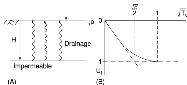
Figure 13 Consolidation.
