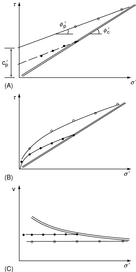
Figure 11 Peak strength.
