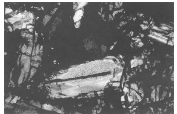
Figure 13 Thin section view of the microtexture of the Nakhla meteorite, a typical achondritic texture resembling that of terrestrial igneous rocks, formed by diopside pyroxene, olivine, and a few plagioclase crystals ( \times 10 ) (from McCall 1999, reproduced with permission of Palgrave Macmillan).
