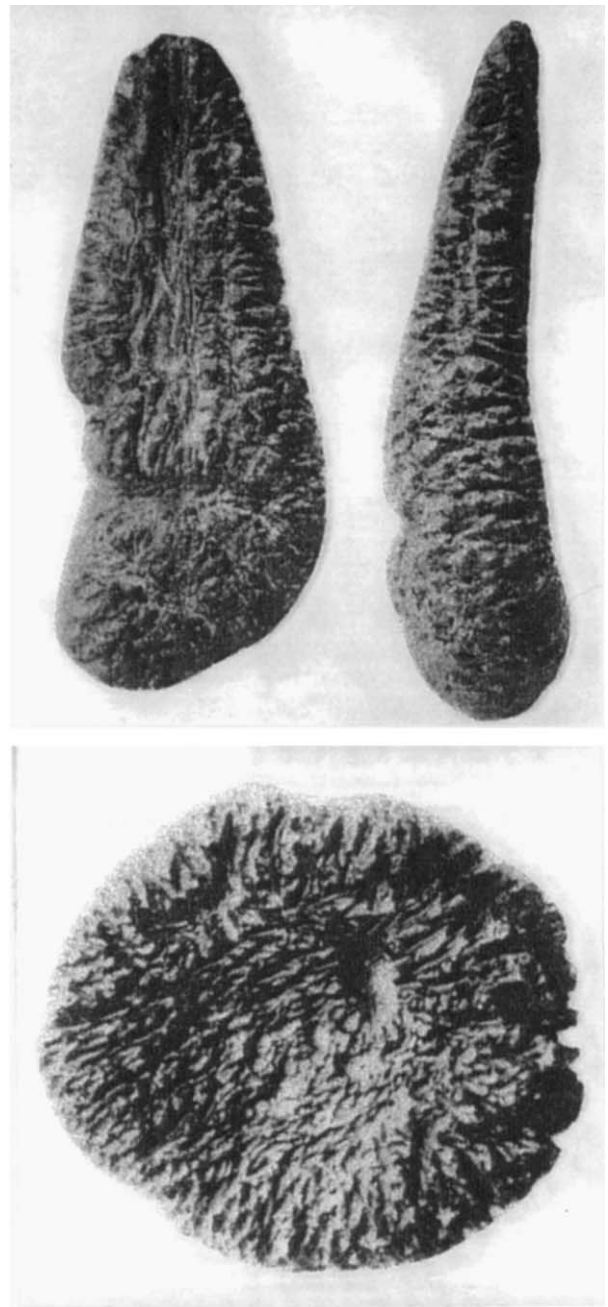
Figure 4 Moldavites from the Czech Republic, showing two teardrops and a discoidal form. Reproduced with permission from McCall GJH (2001) Tektites in the Geological Record: Showers of Glass from the Sky . Bath: Geological Society Publishing House.
