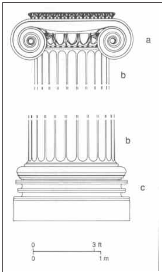
6.17 Ionic capital with spiral scrolls (a); it is supported by a tapering column, greater in circumference at the bottom. The column has deep fluting (b) and stands on a base (c). This type of column stood in the temple of Athena Polias, Priene.
