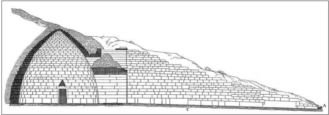
10.12 A cross section through the tomb known as the Treasury of Atreus at Mycenae, with the burial chamber on the left
