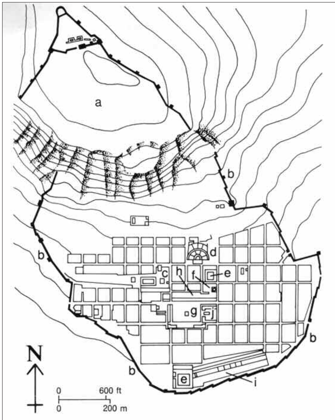
6.2 Town plan of Priene on the slopes of a hill: a) acropolis; b) town walls; c) temple of Athena Polias; d) theater; e) gymnasia (two); f) bouleuterion and prytaneion; g) agora; h) sacred stoa; i) stadium; j) temple of Zeus
