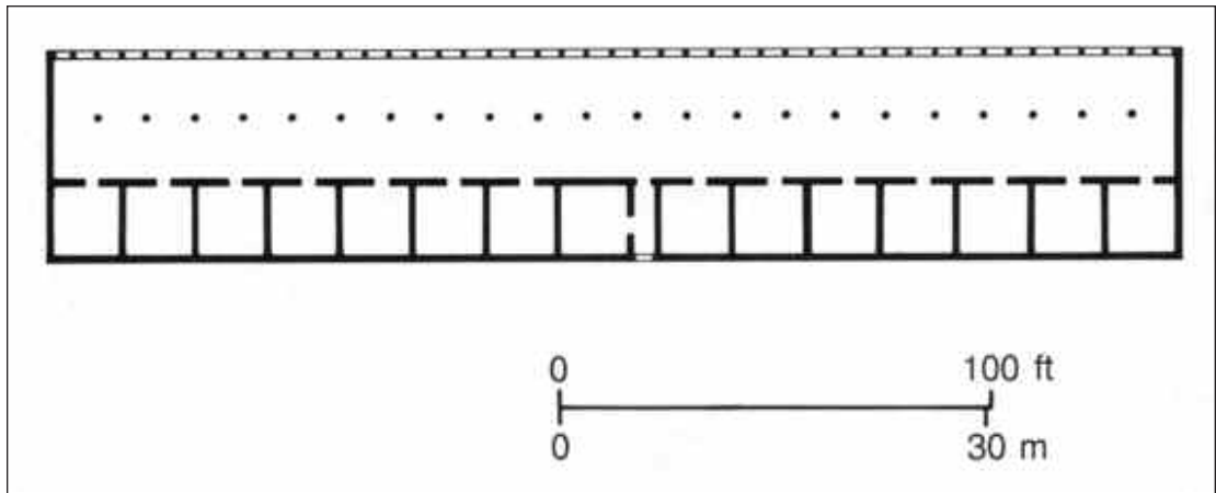
6.9 Plan of South Stoa I in the agora at Athens, which consisted of two rows of columns, a row of rooms and an upper floor. At least two rooms had couches for dining. The stoa was constructed at the end of the 5th century BC.
