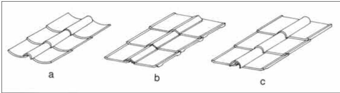
6.28 Types of roof tile: a) Laconian; b) Corinthian; c) Sicilian
