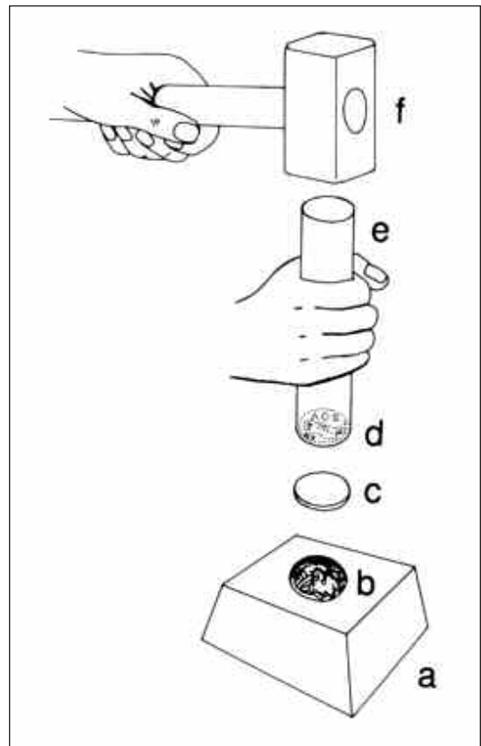
5.12 Striking a coin: a) anvil; b) obverse die; c) coin blank; d) reverse die; e) punch; f) hammer
