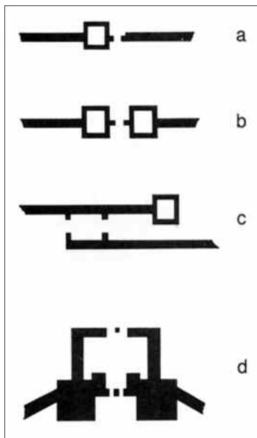
3.19 Plans of fortification gateways dating from the Classical period: a) one flanking tower; b) two flanking towers; c) overlapping type with one tower; d) Hellenistic courtyard type
