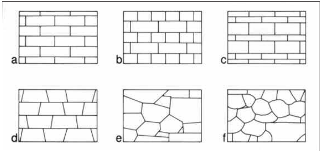
6.27 Types of bond used in masonry construction: a) and b) isodomic (or ashlar); c) pseudoisodomic; d) trapezoidal; e) polygonal; f) Lesbian polygonal
