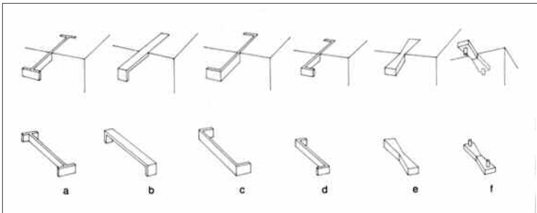
6.26 Types of masonry clamps: a) H-shaped (or double T); b) flat staple (or book); c) U-shaped; d) Z-shaped; e) dovetail (or swallow tail); f) reinforced dovetail
