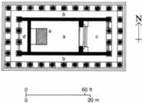
8.31 Plan of the temple of Athena Polias at Priene, dedicated by Alexander the Great: a) cella reached by steps from the porch; b) peristyle; c) deep porch with two columns in antis; d) opisthodomus with two columns in antis; e) pedestal for a cult image. Its architect was Pythius, who wrote a book on this temple.
