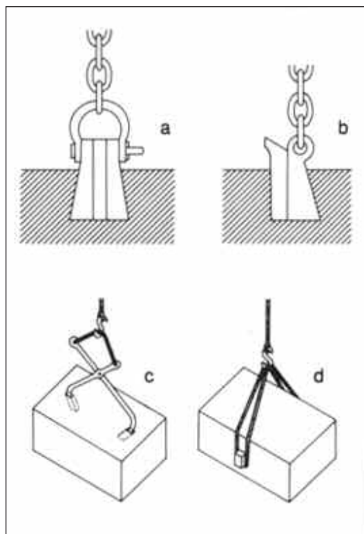
6.23 Methods of lifting masonry blocks: a) lewis iron wedged in a lewis hole attached to an iron chain and pulley system (not shown); b) side view of another shape of lewis iron; c) lifting tongs inserted into holes in a stone block and being hoisted by a rope; d) a stone block being lifted by a sling attached to projecting pieces of stone
