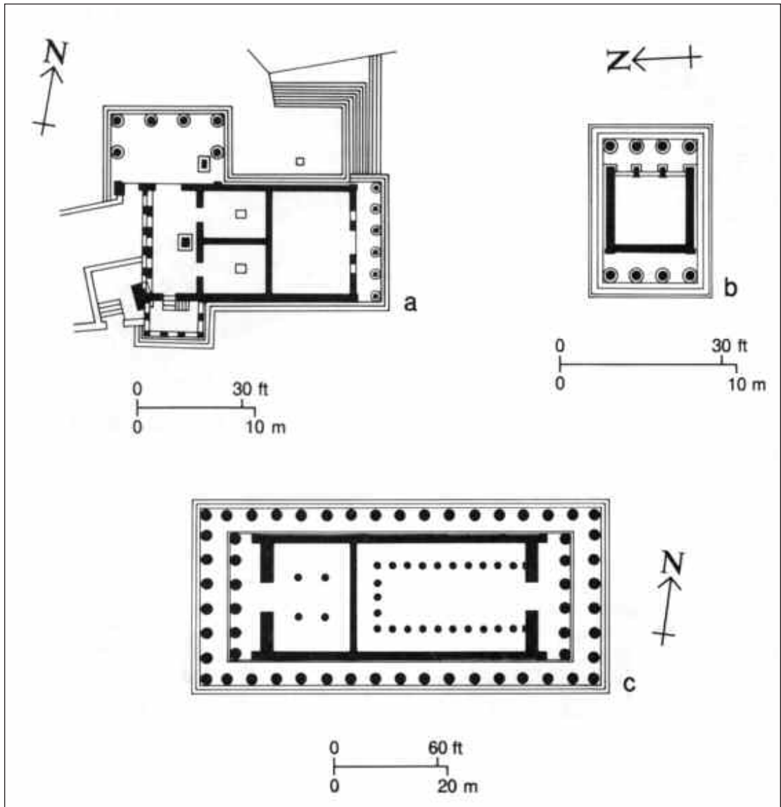
8.28 Plans of temples at Athens: a) Erechtheum; b) Athena Nike; c) Parthenon
